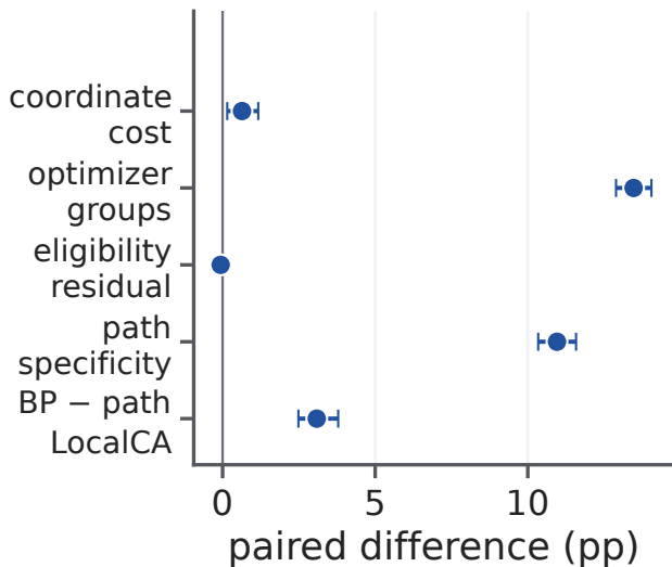
BP-local decomposition
