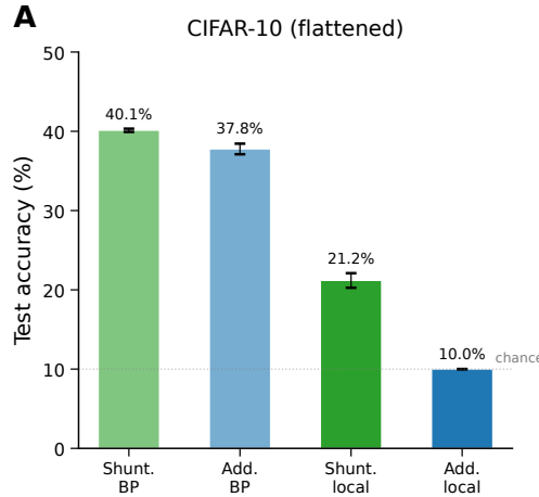
Figure S6: Conservative flattened CIFAR-10 reference sweep . In this appendix stress test, shunting backprop reaches 40.1%, additive backprop 37.8%, shunting local 21.2%, and additive local 10.0% (chance). The backprop–local gap (about 19 pp for shunting) is larger than on MNIST, reflecting the increased difficulty of propagating credit through conductance-based layers for complex visual features. This panel should be read as a conservative flattened-image benchmark rather than as the tuned CIFAR ceiling for the architecture family.
