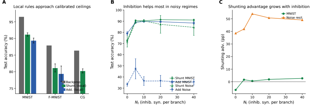
Figure 4: Local competence and regime dependence. (A) Backprop ceiling (gray) vs. best local rule (5F per-soma) for shunting (green) and additive (blue) cores on MNIST, Fashion-MNIST, and context gating. (B) N_I dose-response: test accuracy vs. inhibitory synapses per branch ( N_I ) for shunting and additive cores on MNIST (solid) and noise resilience (dashed). Shunting needs N_I \geq 5 to reach high accuracy; additive learning fails on noise resilience regardless of N_I . (C) Shunting advantage ( \Delta , in percentage points) vs. N_I . The shunting advantage grows with inhibitory synapses per branch and is larger on the noise-resilience task than on MNIST.
