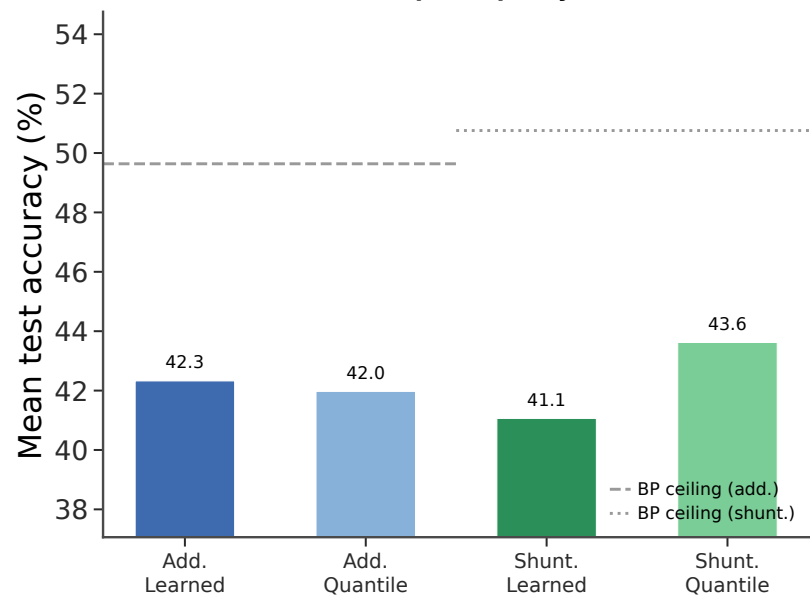
CIFAR-10: LocalCA b,m update policy
