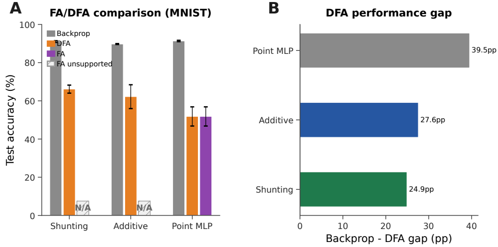
Figure S8: Feedback alignment baselines (MNIST) . (A) Grouped comparison: standard backprop (neutral gray), DFA (orange), and FA (purple). Hatched N/A markers indicate that FA is not implemented for the block-structured dendritic architectures because the random feedback matrices are not dimensionally compatible with the tree-structured branch updates. DFA achieves 66.1% on shunting vs. 62.2% additive vs. 51.8% point MLP. (B) Backprop–DFA gap: dendritic architectures (24.9–27.6 pp) show smaller gaps than point MLPs (39.5 pp), suggesting conductance-based architecture is partially compatible with random feedback.
