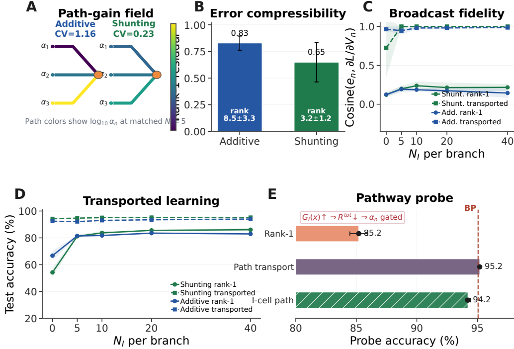
Figure 3: Mechanistic chain from path gains to learning. (A) Example dendritic path-gain field at matched inhibition, with measured MNIST CV annotated for additive and shunting networks. (B) Exact-error compressibility on MNIST: lower rank-1 residual and lower participation rank mean that a scalar broadcast is a better approximation. (C) Direct compartment-error fidelity on noise resilience. Solid lines compare rank-1 broadcast to the exact compartment error; dashed lines show the transported-error oracle. (D) Learning with the transported-error oracle. Improving the broadcast field recovers near-ceiling local learning, especially where rank-1 broadcast fails. (E) Compact inhibitory-path probe. In a one-layer noise-resilience test, exact path transport closes the rank-1 gap, and explicit inhibitory cells trained by the same local rule remain near the explicit-I backprop ceiling. Error bars denote \pm 1 s.d. across seeds.
