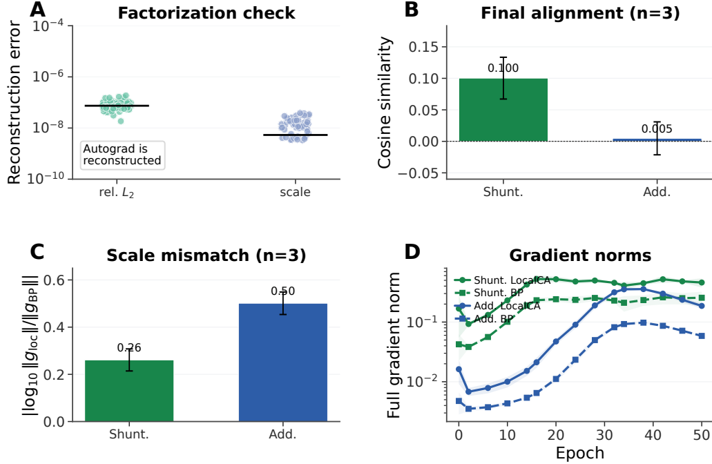
Figure 2: Gradient-fidelity diagnostic. (A) Exact-factorization sanity check across all theory-diagnostic conditions, reported as relative L_2 reconstruction error and scale mismatch. Reconstructed gradients match autograd to numerical precision. (B) Seeded final-checkpoint weighted cosine similarity between local and backprop gradients. (C) Seeded final-checkpoint scale mismatch, defined as |\log_{10}(\|g^{\text{local}}\|/\|g^{\text{BP}}\|)| . Error bars denote \pm 1 s.d. across 3 checkpointed seeds. (D) Full-gradient norms over learning. Additive local and backprop gradients remain finite, so near-zero additive cosine reflects directional mismatch rather than vanishing gradients.
