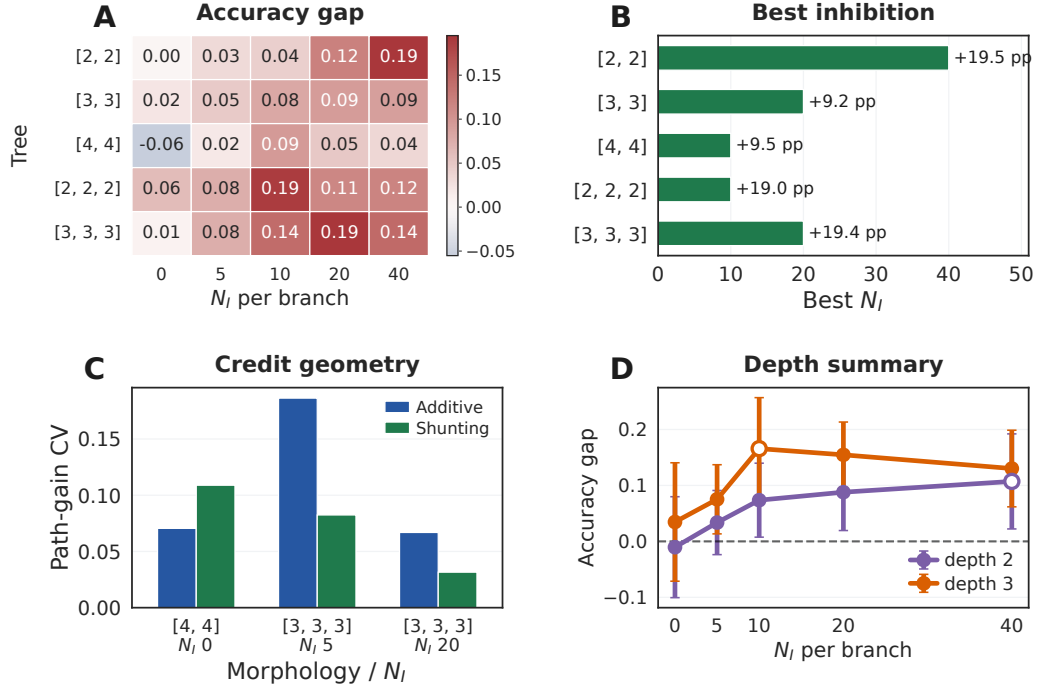
Figure 5: Morphology shifts the useful inhibitory regime. (A) Shunting-minus-additive LocalCA accuracy gap across dendritic morphologies and inhibitory synapse counts. (B) Best inhibitory count for each morphology. (C) Representative path-gain diagnostic for selected morphology cells, used to connect the performance map to credit geometry. (D) Average shunting advantage by depth, with markers showing the peak inhibitory count for each depth.
