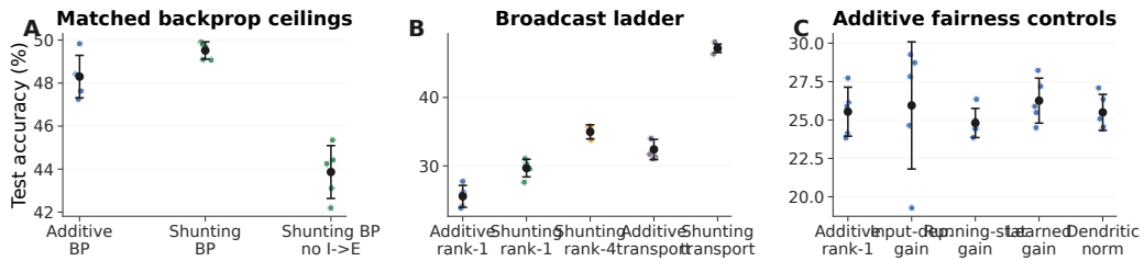
Figure S9: CIFAR-10 control ladder in the compact direct-I-stream family . (A) Matched backprop ceilings. With nonnegative inputs and a nonlinear decoder, shunting slightly exceeds additive under standard training, and removing learned I-to-E conductance lowers the shunting ceiling. (B) Broadcast ladder. Rank-1 broadcast remains weak on this harder dataset, rank-4 improves partially, and exact transported error nearly reaches the shunting backprop ceiling. (C) Additive fairness controls. Input-dependent gain, running-stat gain, learned gain, and dendritic normalization do not rescue additive rank-1 broadcast. This figure is a harder-data diagnostic, not a claim of competitive CIFAR-10 benchmarking.
