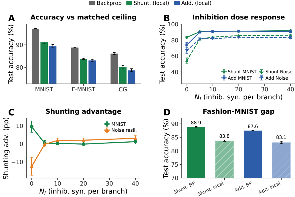
Figure 4: Capacity-calibrated competence and regime dependence. (A) Matched backprop ceilings vs. rank-1 5F LocalCA on MNIST, Fashion-MNIST, and context gating, including the matched additive context-gating rerun. (B,C) Inhibitory dose-response and shunting advantage on MNIST and noise resilience. (D) Fashion-MNIST confirms a smaller but consistent shunting advantage. Error bars denote \pm 1 s.d. across seeds.
