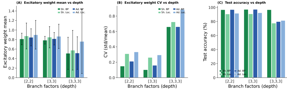
Figure S21: Synaptic weight statistics vs. dendritic depth (MNIST, 5 seeds/cell). (A) Excitatory weight mean (error bars = std). At [2, 2] and [3, 3], all four conditions cluster around 0.8–0.9; at [3, 3, 3] the means drop to \approx 0.5 –0.75 and the cross-seed spread grows, especially for additive LocalCA. (B) Coefficient of variation (CV = std/mean). At shallow/medium depth, LocalCA produces \sim 2\times higher CV than matched BP, but both remain well-behaved ( \leq 0.33 ). At the deepest network all four conditions jump to CV \approx 0.66 –0.88, with additive LocalCA the broadest. (C) MNIST test accuracy. BP tracks \sim 96 –97% at [2, 2]/[3, 3] and \sim 92 –95% at [3, 3, 3]. LocalCA stays within \sim 5 –6 pp of BP at shallow/medium depth but trails by \sim 15 –20 pp at [3, 3, 3], identifying depth as the remaining open challenge for this local rule. The qualitative ordering (shunting LocalCA tracks shunting BP more closely than additive LocalCA tracks additive BP) reinforces the manuscript claim that the conductance denominator is the key mechanistic ingredient.
