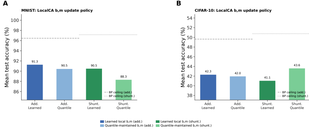
Figure S18: (b, m) update policy under quantile initialization. Each cluster of bars compares the mean test accuracy of learned local (b, m) and quantile-maintained (b, m) under LocalCA for additive and shunting cores, averaged across a matched morphology/init grid ([2, 2] and [3, 3, 3] ; analytical and quantile init variants). Dashed and dotted horizontal lines mark the matched standard backpropagation ceiling for additive and shunting respectively. Left (MNIST): Learned local (b, m) is consistently better; quantile-maintained lags by 1.9 pp (additive) and 3.4 pp (shunting) on mean accuracy. Right (CIFAR-10): The gap reverses for shunting: quantile-maintained reaches 43.6% mean vs. 40.3% for learned local, while additive is essentially tied. The pattern suggests that quantile-maintained (b, m) prevents over-fitting the reactivation gate on harder inputs, making it a useful alternative in harder visual regimes.
