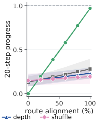
20-step learning
