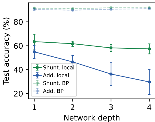
A Depth stress test
