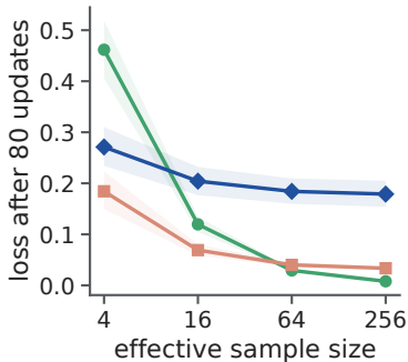
Final-loss crossover
