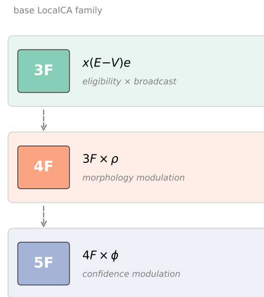
(B) Local learning rule hierarchy
