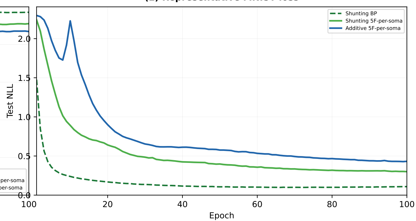
(E) Representative MNIST loss
