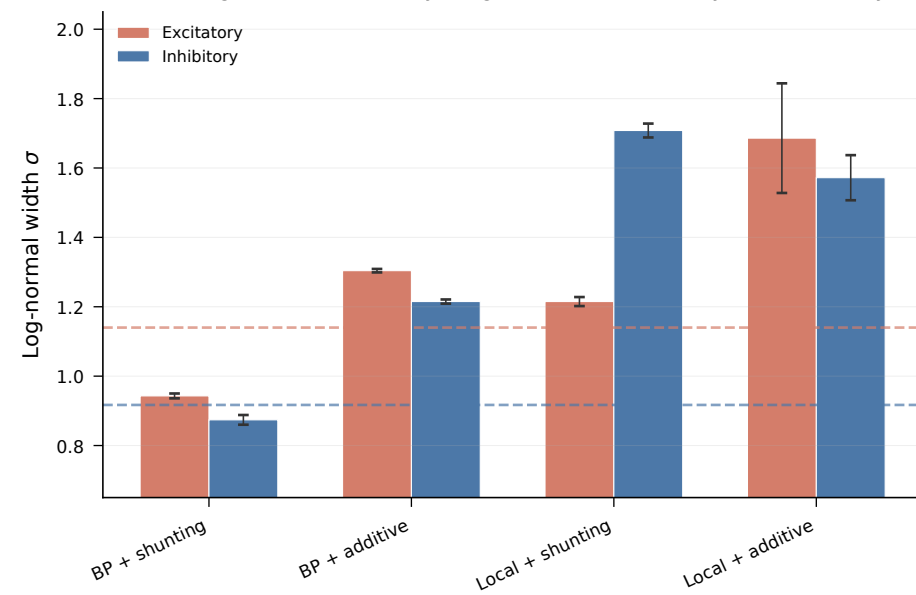
Shunting narrows excitatory weights more consistently than inhibitory
