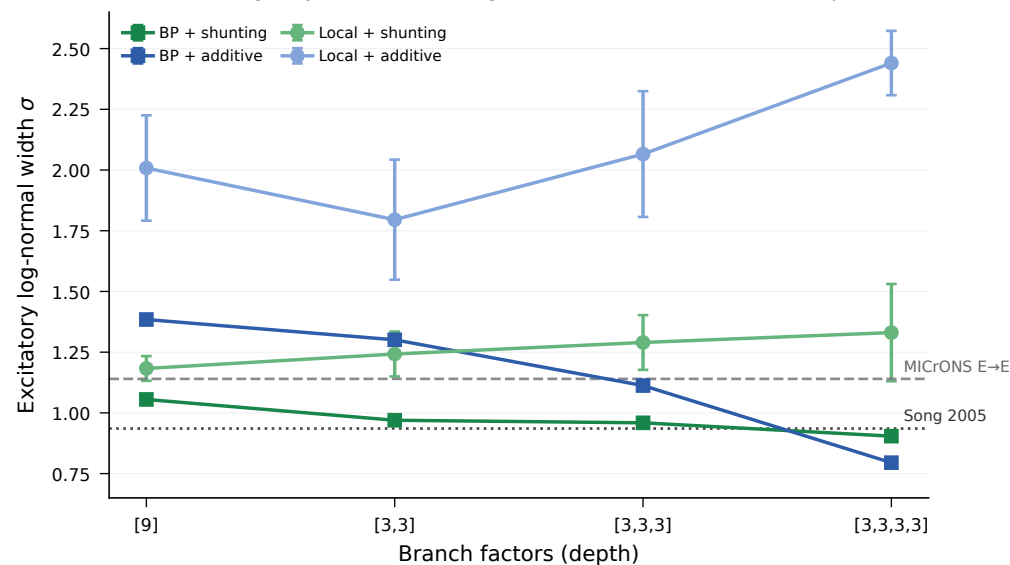
Shunting stays closer to biological-width references across depth
