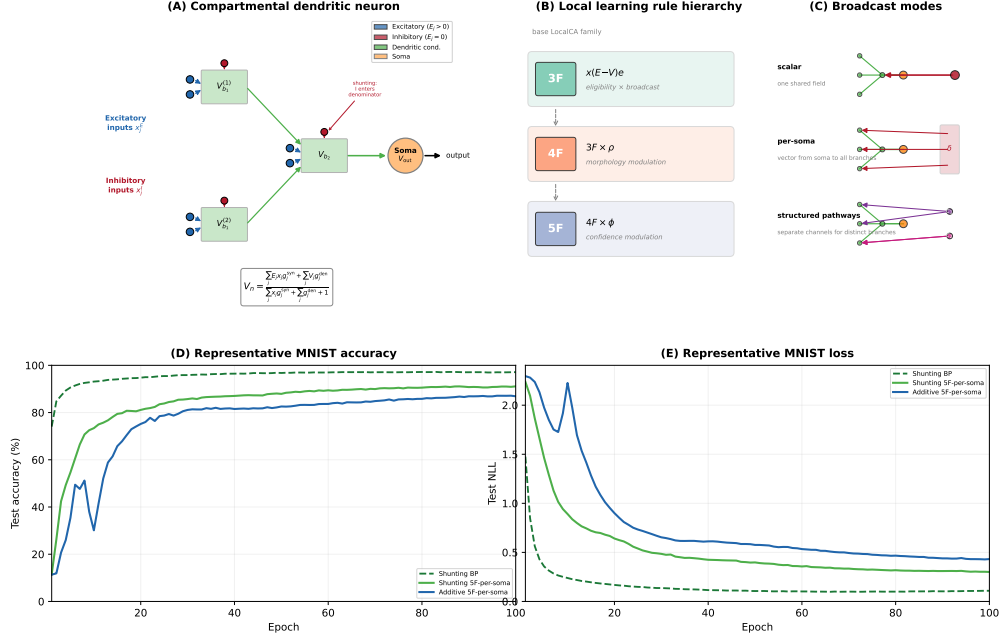
Figure 1: Model and credit assignment. (A) A compartmental dendritic neuron with excitatory (blue triangles) and inhibitory (red circles; shunting) synapses. Voltages propagate to the soma through learned dendritic conductances (green arrows). A somatic broadcast error e_n (dashed red) reaches all compartments; each synapse combines e_n with local quantities (presynaptic drive x_j , input resistance R_n^{\text{tot}} , and driving force E_j - V_n ). (B) Compact LocalCA hierarchy: 3F uses local eligibility and a broadcast field; 4F adds the morphology-aware factor \rho ; 5F further adds the confidence-like factor \phi . (C) Broadcast-mode schematic. Scalar broadcast sends one shared field to all branches; per-soma broadcast sends a vector-valued somatic error to each branch; structured pathway feedback uses separate channels to preserve pathway identity when different branches should receive different teaching signals. (D) Representative MNIST accuracy curves from the current paper configurations, all trained for 100 epochs without early stopping: a shunting backprop reference run reaches 97.1%, shunting 5F-per-soma LocalCA reaches 91.1%, and a matched additive 5F-per-soma LocalCA control reaches 87.1%. (E) The corresponding test negative log-likelihood curves. The revised panels use the current headline configurations rather than the older sandbox trace, and the color scheme matches the rest of the paper: dark green for shunting backprop, green for shunting LocalCA, and blue for additive LocalCA.
