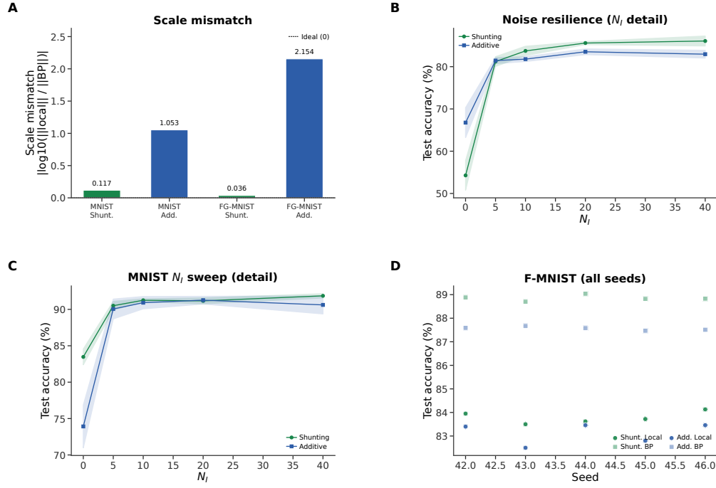
Figure S3: Extended gradient and N_I analysis (supplementary). (A) Log-scale mismatch, |\log_{10}(\|g^{\text{local}}\| / \|g^{\text{bp}}\|)| , from a separate matched-weight static diagnostic; these values should not be compared directly to the checkpointed final-state diagnostic in Fig. 2. The ideal value is 0; shunting is near ideal (0.117), whereas additive shows order-of-magnitude distortion ( > 1.0 ). (B) Noise-resilience N_I dose-response with error bands ( \pm 1 s.d.). (C) MNIST N_I dose-response detail with error bands. (D) Fashion-MNIST individual seeds for all conditions, showing consistency across runs.
