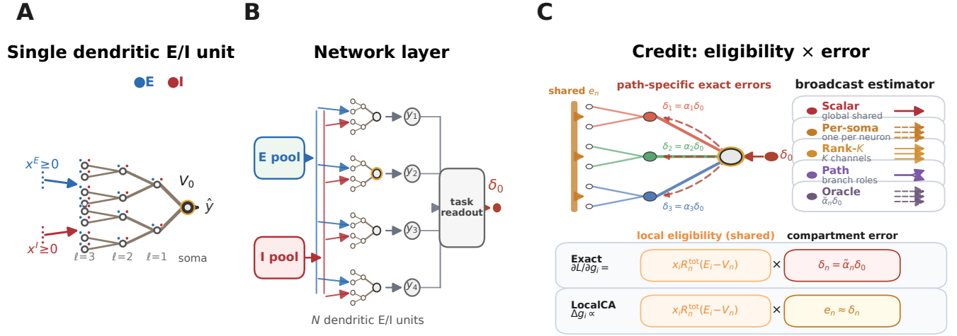
Figure 1: Model and credit assignment. (A) Dendritic E/I unit with branch synapse banks. (B) Layer of such units projecting to a task readout; \delta_0 = \partial L / \partial \mathbf{V}_0 is the soma/core error used for feedback. (C) Exact updates multiply local eligibility by path-specific errors \delta_{u,n} ; LocalCA replaces them with broadcast estimates e_{u,n} of increasing fidelity.
