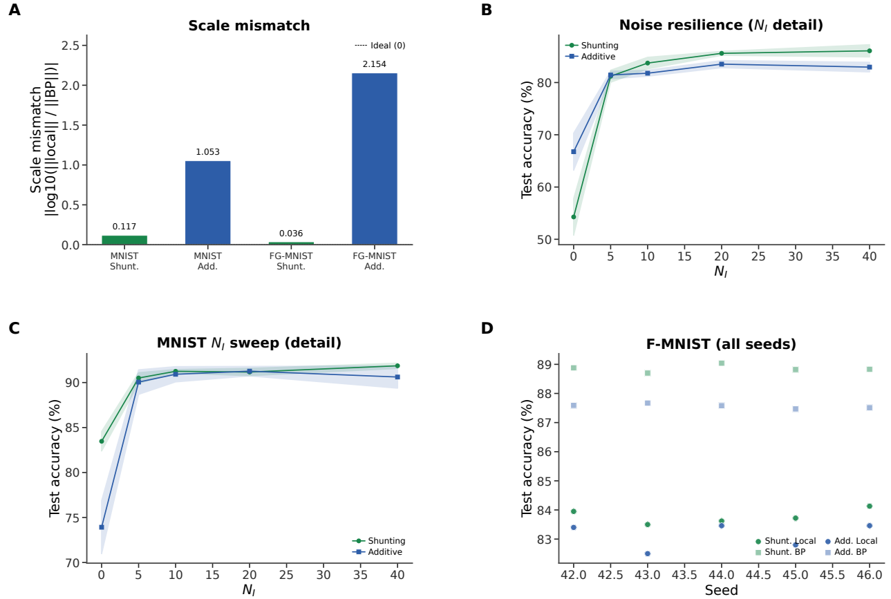
Figure S3: Extended gradient and N_l analysis (supplementary). (A) Log-scale mismatch, |\log_{10}(\|g^{\text{local}}\|/\|g^{\text{bp}}\|)| , from a separate matched-weight static diagnostic; these values should not be compared directly to the checkpointed final-state diagnostic in Fig. 2. The ideal value is 0; shunting is near ideal (0.117), whereas additive shows order-of-magnitude distortion ( > 1.0 ). (B) Noise-resilience N_l dose-response with error bands ( \pm 1 s.d.). (C) MNIST N_l dose-response detail with error bands. (D) Fashion-MNIST individual seeds for all conditions, showing consistency across runs.
