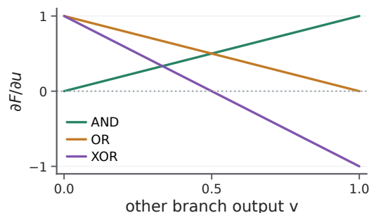
Canonical conditional credit
