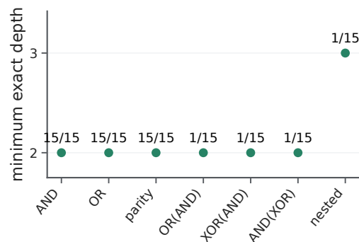
Associative gates are structure controls
