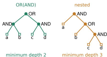
Equal resources; different minimum depth
