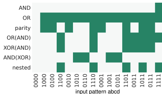
Seven exact Boolean truth tables
