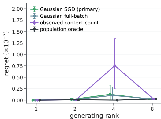
Strong baselines in the joint arm
