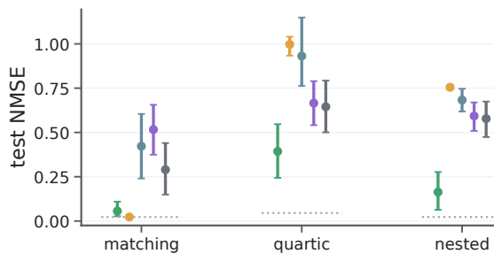
SGD: compatible trees
