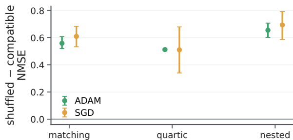
Exact credit: input assignment matters
