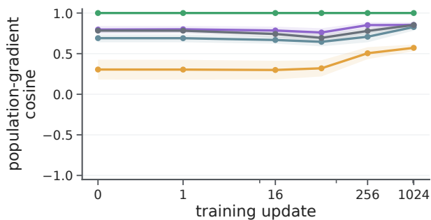
Adam: aggregate gradient alignment
