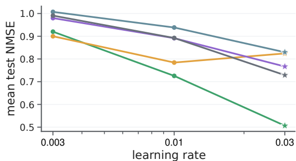
SGD: all learning rates retained
