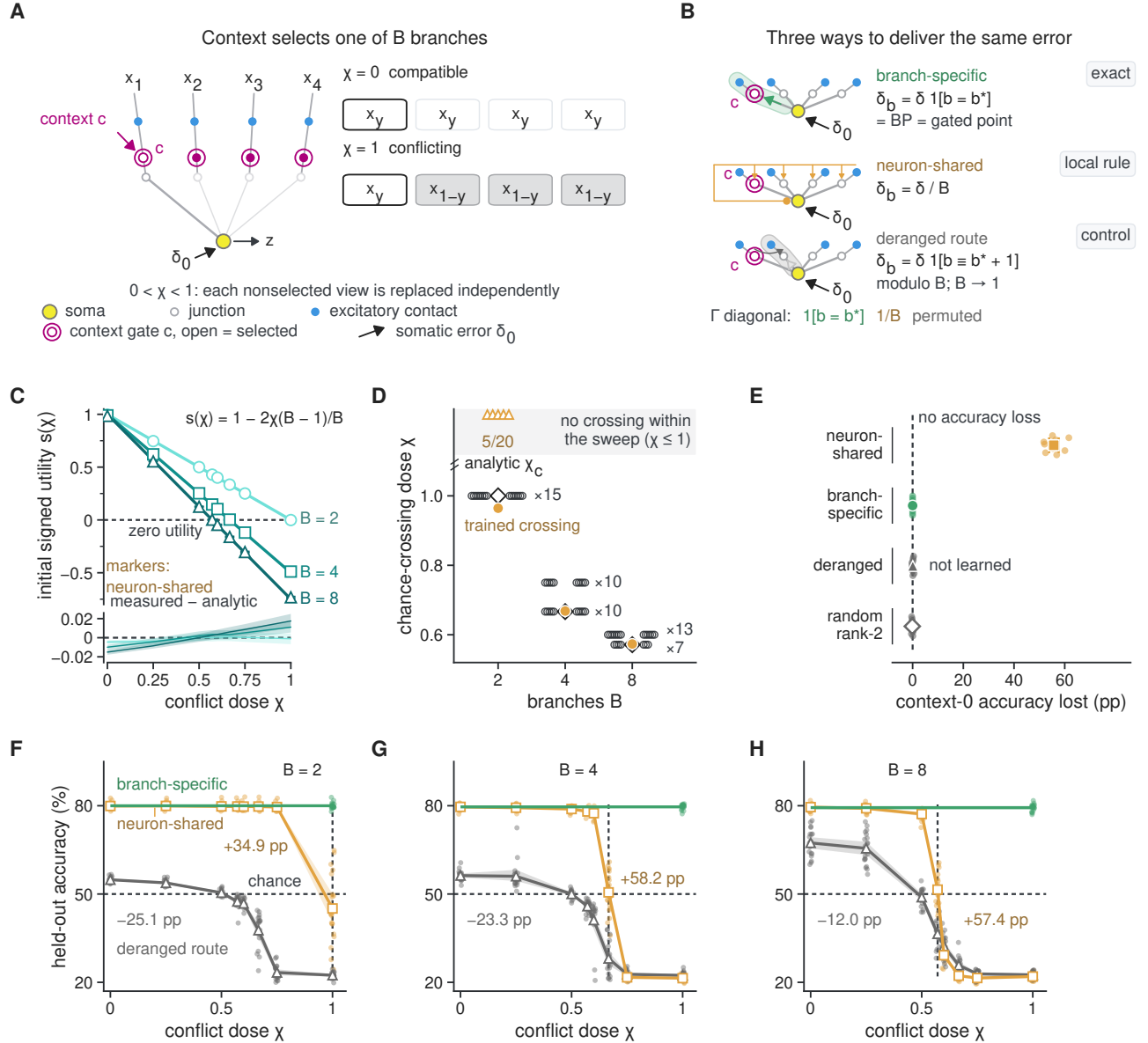
Figure 2: Neuron-shared credit tolerates redundant inputs but fails as branch inputs conflict. A , Context-gated binary branch selection using Fashion-MNIST classes 0 and 6 ( B = 4 schematic). Context selects the branch whose image determines target y ; x_y and x_{1-y} denote target- and opposite-class inputs. Open carmine gate c , selected branch; filled gates and faded stems, inactive branches; ink arrow, \delta_0 . Tiles show conflict doses \chi = 0, 1 . B , Three deliveries on identical fans: branch-specific \delta \mathbf{1}[b = b^*] (green capsule, identical to BP and to a gated point), neuron-shared \delta/B (amber bus, one drop per junction) and a deranged route \delta \mathbf{1}[b \equiv b^* + 1 \pmod B] (grey capsule; cyclic indexing). Branch selection is a diagonal gain \Gamma (Eq. 4). C , Analytic s(\chi) = 1 - 2\chi(B-1)/B (lines; the teal ramp is ordinal in B ) against the neuron-shared rule's measured initial signed utility (open markers). Inset residuals (measured - analytic): hairlines, means; ribbons, 95% intervals; \pm 0.026 scale. n = 20 seeds per cell, mean and 95% seed-bootstrap interval at initialization. D , Analytic \chi_c = B/[2(B-1)] (open ink-edged diamonds) against the trained mean neuron-shared curve's first chance crossing (amber) and each seed's first at-or-below-chance dose ( \times n , seeds at that level); trained crossings 0.964, 0.668 and 0.573 (exact two-sided sign test on the predicted order, P = 1.9 \times 10^{-6} ). The strip above the axis break holds five B = 2 non-crossing seeds; n = 20 seeds per B , sweep levels without intervals, endpoint state. E , Separate synthetic two-stream task: context-0 accuracy loss after mixed-context acquisition and context-1-only training. Routes: neuron-shared (amber square), branch-specific (green circle), deranged (grey filled triangle) and a random dense rank-2 field (grey open diamond); faint dots, individual seeds; branch-specific minus neuron-shared -55.7 [ -57.7, -53.8 ] points, paired Wilcoxon P = 0.002 . Deranged routing never learned (held-out 19.6%); its near-zero accuracy loss does not indicate memory retention. Depth-shared equalled neuron-shared in every seed and is not drawn. n = 10 paired seeds, mean and 95% seed-bootstrap interval. F-H , Held-out accuracy against \chi at B = 2, 4 and 8 for B 's three deliveries; dashed vertical, \chi_c ; dashed horizontal, binary chance (50%); faint dots, seeds. Branch-specific accuracy is \chi -invariant by construction (one line, band and seed fan). Grey tags, deranged - branch-specific at \chi = 0 ; amber tags, branch-specific - neuron-shared at \chi = 1 . n = 20 paired seeds, mean and 95% seed-bootstrap band at the endpoint. Source Data: source_data/curated_publication/figure_02_plotted.csv .
