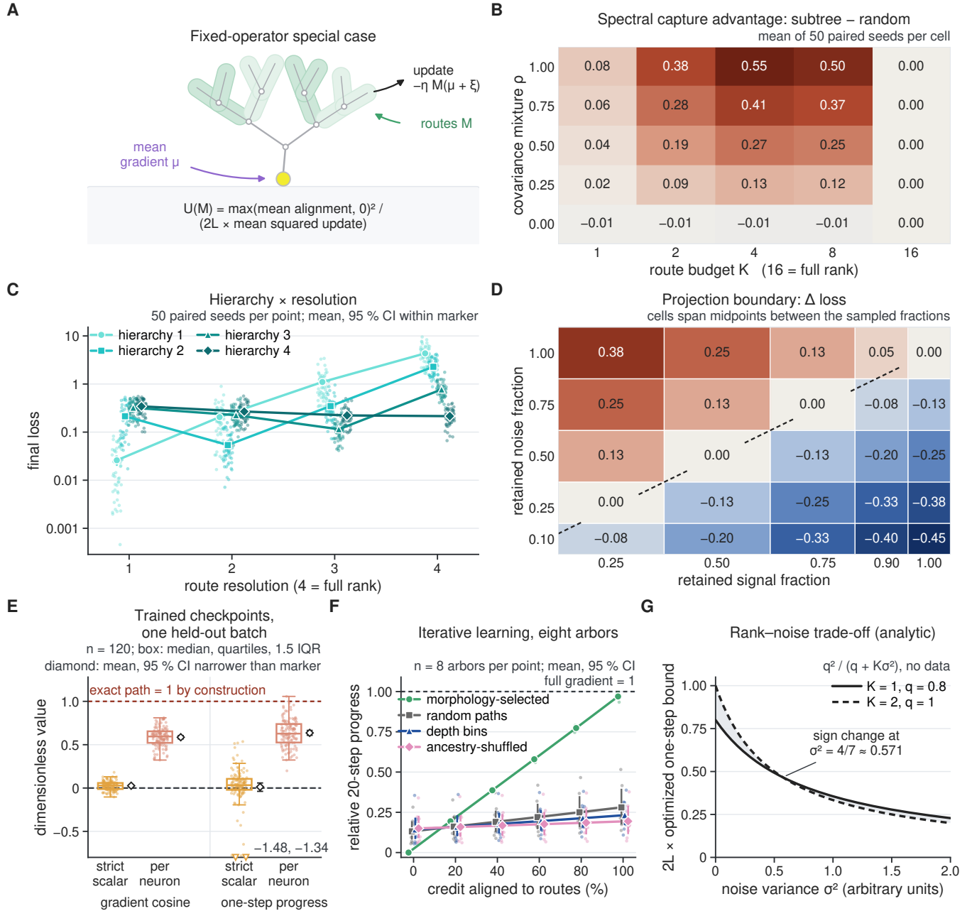
Figure S3: Signal retention and noise jointly constrain one-step progress. Dots show individual units; large symbols, means and 95% bootstrap intervals ( C , seeds; E , checkpoints; F , cells, one Monte Carlo stream each). Intervals in C,E lie under markers. B,D colour printed cell values by sign (red positive, blue negative) and magnitude; B 's -0.01 controls are near-neutral. A , Fixed-operator one-step guarantee: U(M) = \max(\mu^\top M \mu, 0)^2 / (2LE\|M(\mu + \xi)\|^2) ( \xi , zero-mean noise; L , loss smoothness) lower-bounds the expected decrease at the bound-optimal nonnegative step \eta^* , subject to smoothness along the update segments (Eqs. 42,43); zero updates have U = 0 . B , Subtree-minus-random spectral capture over route budget K and covariance mixture \rho , 50 paired seeds per cell; K = 16 and \rho = 0 are by-construction controls, only the endpoints isospectral. C , Final loss against route resolution D_r for hierarchies H_c = 1-4 (teal, light to dark; circle, square, triangle, diamond); D_r = 4 resolves every leaf ( M = I ); 50 paired seeds per point, series dodged in x . D , Exact projection boundary: retaining signal fraction f_{\text{sig}} and noise fraction f_{\text{noise}} changes normalized loss by (f_{\text{noise}} - f_{\text{sig}})/2 ; cell centres are the sampled fractions; the dashed boundary is f_{\text{noise}} = f_{\text{sig}} . E , Gradient cosine and norm-matched progress at 120 trained checkpoints (one held-out batch; relative step 10^{-5} ): strict scalar amber, per neuron salmon. Two below-range scalar values are labelled at the floor. Boxes show medians, quartiles and 1.5-interquartile-range whiskers; open diamonds, means. Dashed references: exact path (dark red, 1), zero (grey). F , Eight-arbor positive control: twenty-step projected loss reduction relative to the full gradient (dashed, 1), with route-aligned credit (green circles, morphology-selected; grey squares, random paths; blue triangles, depth bins; pink diamonds, ancestry-shuffled). G , Analytic rank–noise trade-off, 2L times the optimized bound q^2/(q + K\sigma^2) for (K, q) = (1, 0.8) (solid) and (2, 1) (dashed), both black, crossing at \sigma^2 = 4/7 ; grey shading separates them. E diagnoses actual trained checkpoints; F imposes route alignment and uses oracle projections. Neither tests biological credit or long-horizon selection; endpoint selection fails prospectively (Fig. S34).
