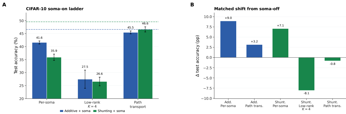
Figure S8: CIFAR-10 compact E/I depth-4 with somatic_synapses=true. (A) Absolute soma-on ladder on the compact explicit-E/I depth-4 family. Path transport stays strongest in both cores and remains near the matched backprop ceilings (dashed lines), while low-rank K=4 remains weak. (B) Matched shift from soma-off to soma-on for the conditions with a clean paired baseline. Soma helps additive strongly under per-soma and path transport, improves shunting per-soma, leaves shunting transported error close to its soma-off value, and worsens shunting low-rank K=4 . Additive low-rank K=4 is omitted from panel B because the corrected soma-off strong-family mechanism package did not include that exact matched rerun.
