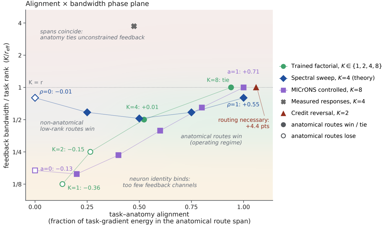
Figure 8: Alignment and bandwidth organize the experimental boundary. O, Task–anatomy alignment is the fraction of task-gradient energy inside the anatomical route span; normalized bandwidth is K/r_{\text{eff}} , where r_{\text{eff}} = (\sum_i \lambda_i)^2 / \sum_i \lambda_i^2 . Markers place the trained subtree factorial, the spectral phase sweep, the controlled MICrONS alignment test, the measured-response null and the two-stream credit-reversal task on the same plane. Labels report ancestry-minus-best-control endpoints; filled markers indicate a win or tie and open markers a loss. Shaded regions summarize credit-operator regimes and are conceptual boundaries rather than fits to the displayed outcomes. Exact coordinates and display offsets are in Source Data.
