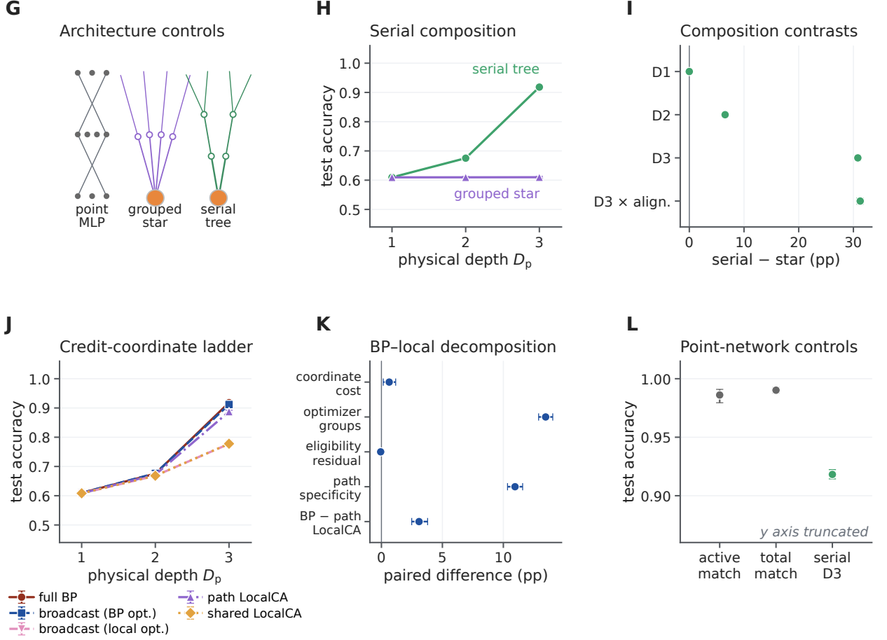
Figure 5: Point-dendrite and BP-local-credit controls. G , Same-task architecture ladder; all controls share the task and paired seeds without retuning. H , Serial tree and exact-resource grouped-star accuracy across physical depth. I , Paired serial-minus-star contrasts and the D3 alignment interaction. J , Full BP, soma-broadcast autograd under the BP or LocalCA optimizer, and shared- or path-transport LocalCA. K , Paired D3 decomposition: teaching-coordinate cost and the optimizer contrast use soma-broadcast autograd; the eligibility residual compares optimizer-matched broadcast with shared LocalCA; path specificity compares the two LocalCA transports. L , Point MLPs matched to active or total parameters versus the serial D3 tree; points show mean accuracy with 95% intervals on a truncated y axis. Means and paired contrasts use the same ten seeds 10200–10209; error bars are 95% seed-bootstrap intervals. The optimizer-matched amendment is post-outcome and diagnostic.
