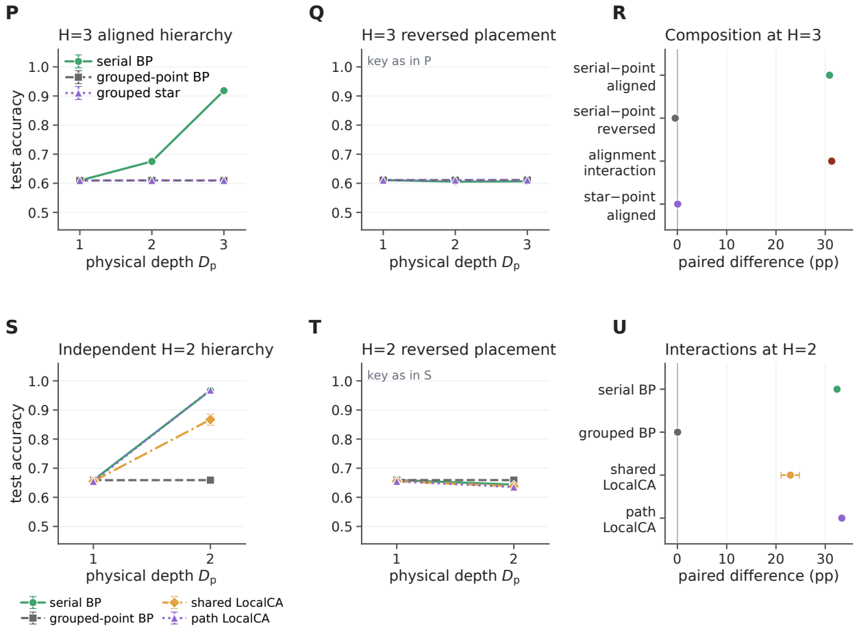
Figure 5: Serial composition replicates across two task hierarchies and vanishes in literal grouped-point controls. P,Q , Existing H = 3 serial tree, literal grouped-point emulation and earlier grouped star under aligned and reversed placement. R , Paired H3 serial-minus-point contrasts, their alignment interaction and the grouped-star-minus-point comparison. S,T , Fresh H = 2 serial BP, grouped-point BP and serial LocalCA with a shared-soma or exact-path coordinate under aligned and reversed placement. U , Paired aligned-minus-reversed D2-minus-D1 interactions. Lines are means across ten paired seeds; all error bars are 95% seed-bootstrap intervals. The H = 2 cohort changes hierarchy and inventory within the same calibrated synthetic task family and is not an independent dataset.
