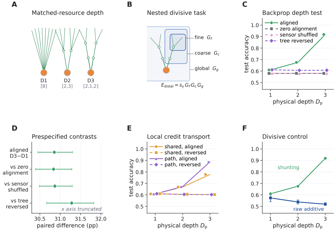
Figure 5: Matched nonlinear hierarchy makes exact-resource physical dendritic depth useful. A , D1–D3 have D_p = 1, 2, 3 stages. Bracket entries are soma-to-distal branching factors: [8] , [2, 3] and [2, 1, 2] give 8, 2 + 6 and 2 + 2 + 4 nonsomatic branch units, with identical contact, candidate-slot, parameter and state budgets. B , A distal positive-rate signal is multiplied by fine, coarse and global gains; independent sensors, trial-shuffled sensors and reversed physical placement are matched controls. C , Test accuracy under shunting backpropagation. Lines in C , E , F are ten-seed means and error bars 95% seed-bootstrap intervals; coincident flat-control markers are offset. D , Prespecified paired D3-minus-D1 effect and aligned-minus-control interactions; bars are 95% paired-seed bootstrap intervals, all excluding zero. E , Aligned and reversed-placement local credit assignment (LocalCA) with one shared-soma coordinate or exact path transport; the coincident reversed curves are drawn with offset markers. F , Aligned shunting and raw-additive BP. All inferential runs use fresh seeds 10200–10209.
