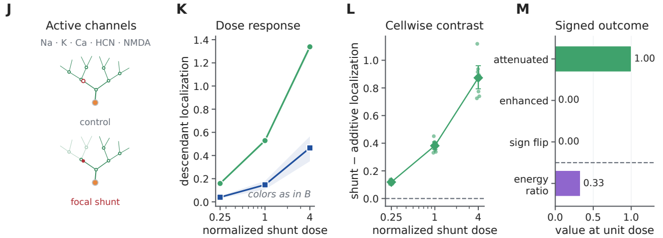
Figure 7: The focal localization signature survives an active-conductance steady-state extension. J , Na, K, Ca, HCN and NMDA conductances were sampled 64 times within each of eight reconstructed cells; every nonlinear equilibrium was solved before evaluating its exact local Jacobian. All draws used R_m = 1,000 \Omega \text{cm}^2 with one baseline-leak unit of distributed background conductance. K , Descendant localization across input-conductance-normalized doses for focal shunting and state-matched additive input. L , Paired shunt-minus-additive localization; small points are reconstructed-cell means after averaging channel draws and focal sites. M , Descendant-gradient outcomes at unit dose: attenuation fraction, enhancement fraction, sign-flip fraction and post-shunt-to-baseline energy ratio. Lines and bands in K and intervals in L are means and 95% cell-bootstrap intervals. Channel draws and sites are nested sensitivities; reconstructed cells are the units of inference.
