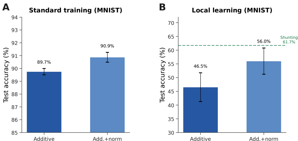
Figure S10: Additive + normalization control (MNIST) . (A) Standard backprop: normalization provides a small boost (89.7% \rightarrow 90.9%). (B) Local learning: normalization improves additive from 46.5% to 56.0% (+9.5 pp), partially closing the gap to shunting (61.7%, dashed green). The remaining gap ( -5.7 pp) indicates that shunting provides benefits beyond simple voltage normalization.
