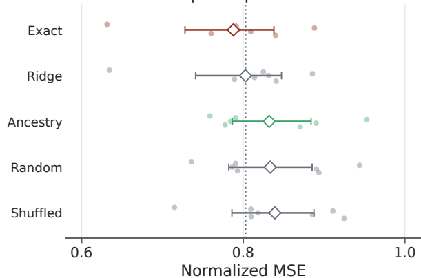
Response prediction
