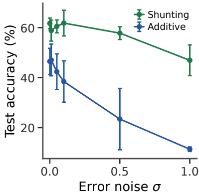
B Broadcast noise
