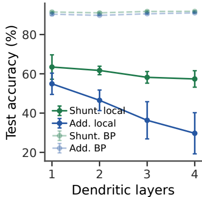
A Depth scaling
