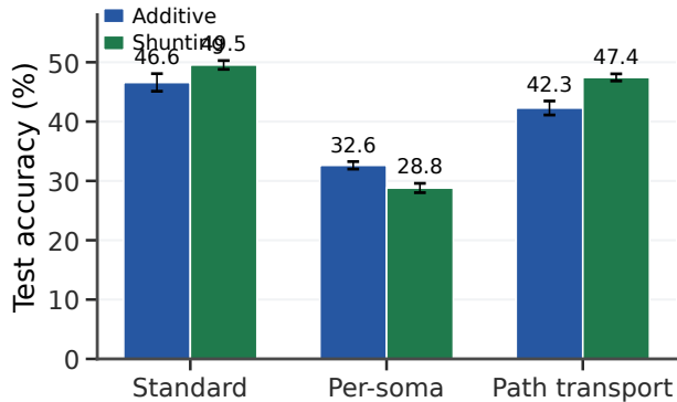
A CIFAR-10 mechanism ladder
