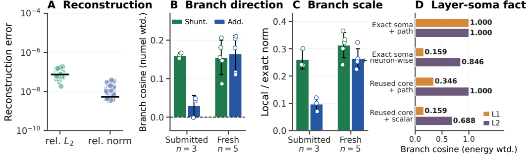
Figure 2: Exact reconstruction and gradient diagnostics. (A) Exact-factorization reconstruction against autograd: relative L_2 error and relative norm error, one point per parameter tensor. (B,C) Matched 3F parameter-count-weighted branch-gradient cosine and local/exact norm ratio at non-somatic dendritic blocks for the three submitted checkpoint pairs and a fresh five-seed cohort; each dot is one checkpoint averaged over train, validation, and test diagnostic batches. Full values and inference limits are reported in Appendix Tables S9 and S10. (D) Energy-weighted branch-gradient cosine in a layer-soma factorial separating exact vs. reused soma teaching signals, neuron-wise feedback, and exact path transport; L1 and L2 denote dendritic network layers. The two L1 conditions shown as 0.159 differ before rounding. Metrics/protocol: Appendix A. Error bars in (B,C) are \pm 1 s.d. across seeds within each cohort.
