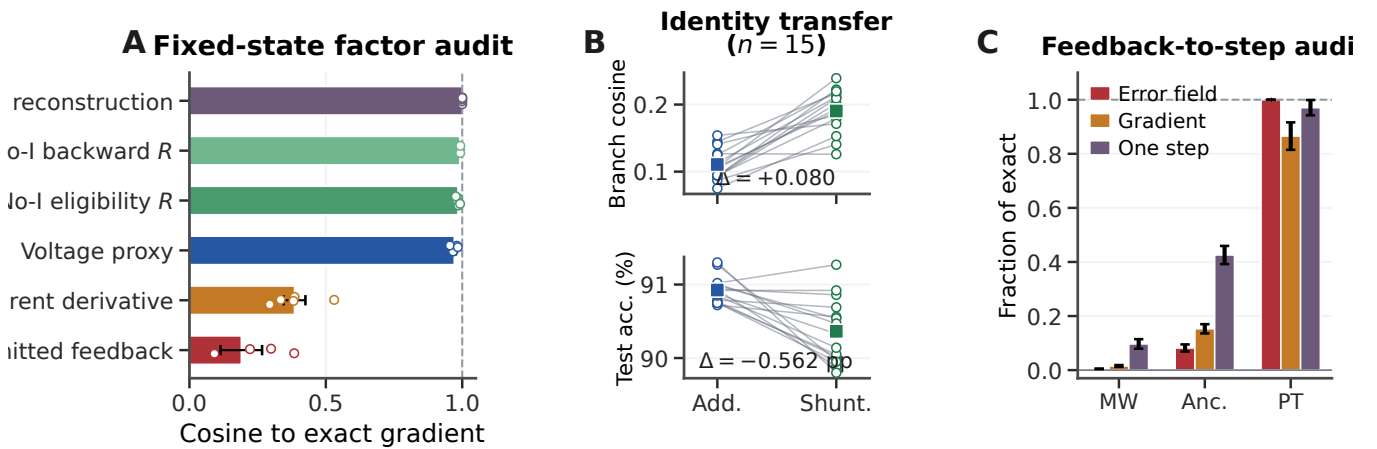
Figure S3: Mechanistic audit separating path effects from learning consequences. (A) Fixed-forward-state factor substitutions in five shunting checkpoints. Removing inhibitory conductance from either resistance factor leaves gradient direction close to exact reconstruction, whereas omitting parent transfer derivatives or using the submitted feedback causes larger directional errors. Bars are mean \pm s.e.m.; points are seeds. (B) Fifteen paired identity-transfer checkpoints. Shunting improves branch-gradient direction, while additive test accuracy remains slightly higher; squares denote means. (C) The same-batch feedback ladder measured as optimally rescaled dendritic error-field capture, eligibility-weighted branch-gradient capture, and norm-matched one-step progress at relative step 10^{-5} . Bars pool five checkpoints per core after averaging three diagnostic splits; error bars are s.e.m. over checkpoints. In this cohort the global scalar equals the submitted field, and the available ancestry field equals exact-soma ancestry. Error geometry alone is therefore not treated as a learning metric. Fixed-state substitutions are diagnostic hybrids, not separately trained forward models.
