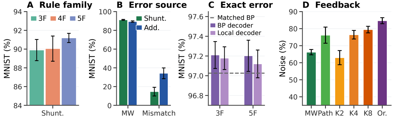
Figure 5: Rule and feedback controls identify the principal learning bottleneck. (A) Within-shunting submitted-code comparison of 3F, 4F, and 5F under matched feedback, decoder, optimizer, and effective parameter-group rates ( n=3 ; descriptive). (B) Error-source negative control under the same local decoder: matched-width/scalar-fallback feedback (MW) supports learning, whereas a compartment-local mismatch does not ( n=3 ); the cross-core ordering is not interpreted. (C) Five-seed exact-transport factorial: 3F and 5F both approach matched backpropagation with either a backpropagated or locally updated decoder; note the ordinate spans only 0.9 percentage points. (D) Noise-resilience feedback ladder: MW, recursive Path, random low-rank K2/K4/K8, and transported Oracle. Together, the panels show that the feedback field, rather than a failure of the local eligibility factorization, sets the dominant practical limit. Error bars are \pm 1 s.d.
