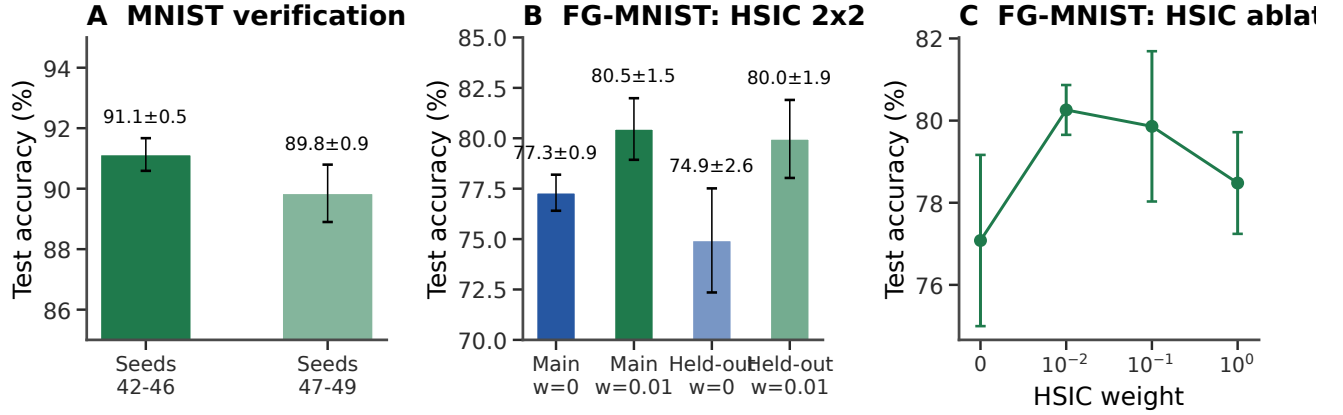
Figure S5: Verification and seed robustness (supplementary). (A) MNIST verification: repeat runs on main seeds (42–46) yield 91.1 \pm 0.5\% ; held-out seeds (47–49) yield 89.8 \pm 0.9\% , showing robustness across random seeds. (B) Matched figure-ground MNIST HSIC control: both main seeds (42–46) and held-out seeds (47–49) compare HSIC weight 0 against 0.01. (C) HSIC weight ablation on figure-ground MNIST: moderate weights (0.01–0.1) perform best.
