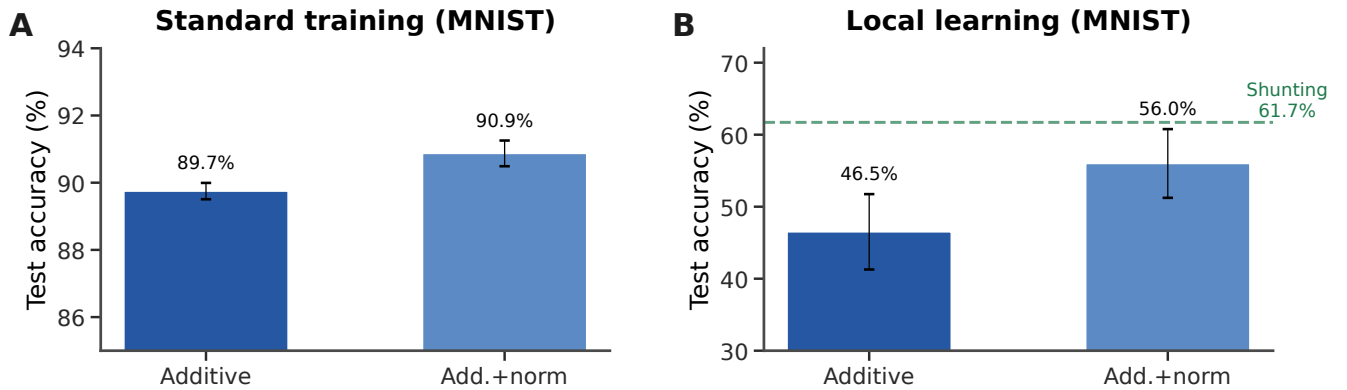
Figure S9: Additive + normalization control (MNIST stress-regime diagnostic). (A) Standard backprop: normalization provides a small boost (89.7% → 90.9%). (B) Local learning: normalization improves additive from 46.5% to 56.0% (+9.5 pp), partially closing the gap to shunting (61.7%, dashed green). These lower local accuracies come from a separate stress-regime diagnostic, not from the matched-capacity performance setting in Table S8.
