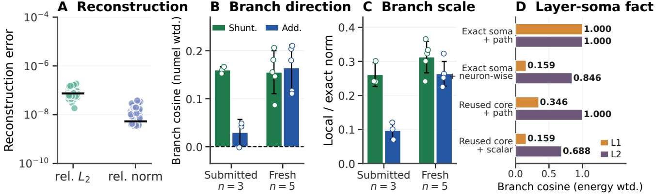
Figure 2: Exact reconstruction and gradient diagnostics. (A) Exact-factorization reconstruction against autograd: relative L_2 error and relative norm error, one point per parameter tensor. (B,C) Matched 3F parameter-count-weighted branch-gradient cosine and local/exact norm ratio at non-somatic dendritic blocks for the three submitted checkpoint pairs and a fresh five-seed cohort; each dot is one checkpoint averaged over train, validation, and test diagnostic batches. Full values and inference limits are reported in Appendix Tables S9 and S10. (D) Energy-weighted branch-gradient cosine in a layer-soma factorial separating exact vs. reused soma teaching signals, neuron-wise feedback, and exact path transport; L1 and L2 denote dendritic network layers. The two L1 conditions shown as 0.159 differ before rounding. Metrics/protocol: Appendix A. Error bars in (B,C) are \pm 1 s.d. across seeds within each cohort.
