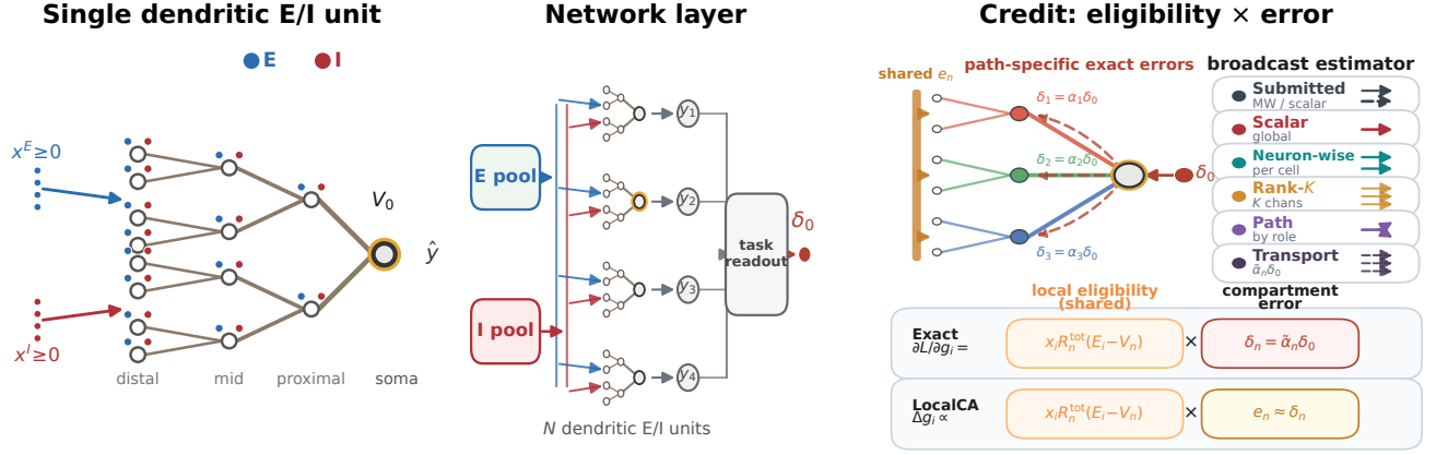
Figure 1: Model and credit assignment. (A) Schematic dendritic unit with excitatory and inhibitory inputs on each branch. (B) Layer of such units projecting to a task readout; \delta_0 = \partial L / \partial V_0 is the soma/core error used for feedback. (C) Exact updates multiply local eligibility by path-specific errors \delta_{u,n} ; LocalCA replaces them with broadcast estimates e_{u,n} . The submitted matched-width/scalar-fallback hybrid is shown separately from strict scalar, neuron-wise, low-rank, path-structured, and transported feedback.
