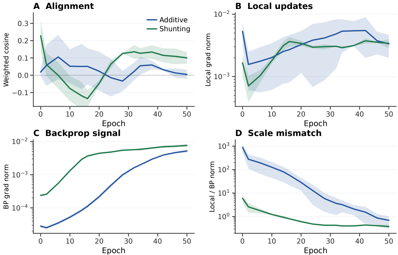
Figure S4: Alignment dynamics with explicit gradient-norm checks. (A) Weighted cosine similarity between LocalCA and backpropagation gradients over training for the 5F rule. (B,C) Weighted local and backprop gradient norms stay nonzero for both additive and shunting models. (D) The additive control begins with a much larger scale mismatch, then approaches the backprop scale without recovering strong directional alignment. Shading is s.d. across 3 seeds.
