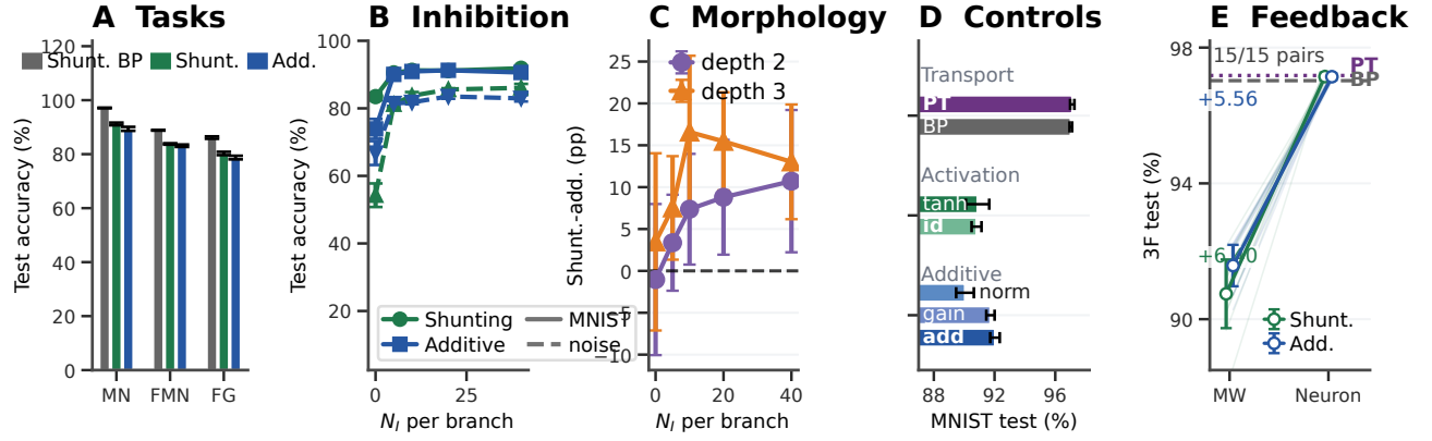
Figure 4: Matched-capacity performance, regime dependence, and feedback correction. (A) Matched shunting backpropagation reference (grey, labelled Shunt. BP) vs. matched-width/scalar-fallback 5F LocalCA; MN, FMN, and FG denote MNIST, Fashion-MNIST, and figure-ground MNIST. Additive backpropagation references are reported in Table S8 where matched five-seed runs are available. (B) Inhibitory dose-response. (C) Descriptive morphology-by-inhibition performance; the detailed map and its initialization limitation are in Appendix Fig. S10. (D) MNIST controls: backpropagation (BP), exact path transport (PT), identity vs. learned tanh activation, and additive gain/normalization variants. (E) Fifteen-seed 3F intervention: replacing matched-width/scalar-fallback feedback (MW) by one neuron-indexed coordinate shared within each modeled tree raises accuracy by 6.40 points in shunting and 5.56 points in additive networks; all paired seeds improve. Dashed and dotted lines mark the matched shunting BP and exact-transport references. Values/protocols: Table S8; Appendix A. Error bars denote \pm 1 s.d.
