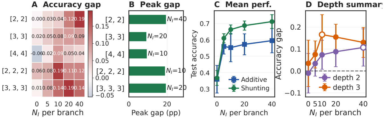
Figure S10: Descriptive morphology × inhibition performance map. (A) Shunting-minus-additive LocalCA accuracy gap across dendritic morphologies and inhibitory synapse counts. (B) Best inhibitory count for each morphology. (C) Mean performance across tested trees. (D) Average shunting advantage by depth, with markers showing the peak inhibitory count for each depth. The grid uses nonnegative inputs. Because analytical initialization places one shunting population at a near-zero coupling floor, these comparisons are descriptive rather than a causal morphology intervention.
