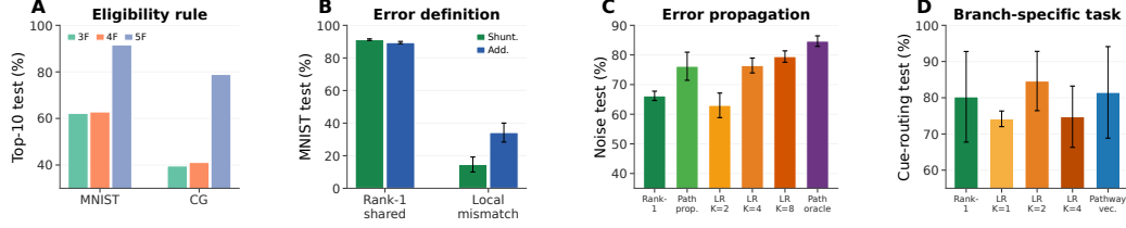
Figure 3: Local-rule and feedback-design axes. (A) The theorem-facing 3F update and the 4F attenuation proxy are weak practical optimizers in the completed local-competence sweeps; 5F is the strongest empirical wrapper. (B) The broadcast definition matters: on MNIST, rank-1 shared somatic error is strong, while a local-mismatch error surrogate fails. (C) On noise resilience, recursively propagating or increasing the rank of the error field closes much of the gap between rank-1 broadcast and exact path transport. (D) Cue routing probes a branch-specific regime: higher rank helps, while the current pathway-vector implementation is useful but not yet better than the best unstructured low-rank control. Error bars denote \pm 1 s.d. where five-seed summaries are available.
