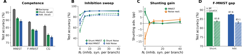
Figure 5: Capacity-calibrated competence and regime dependence. (A) Matched backprop ceilings vs. rank-1 5F LocalCA on MNIST, Fashion-MNIST, and context gating, including the matched additive context-gating rerun. (B,C) Inhibitory dose-response and shunting advantage on MNIST and noise resilience. (D) Fashion-MNIST confirms a smaller but consistent shunting advantage. Error bars denote \pm 1 s.d. across seeds.
