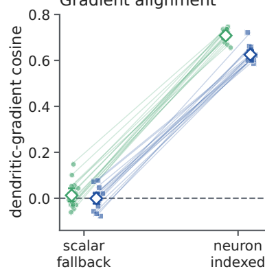
Gradient alignment
