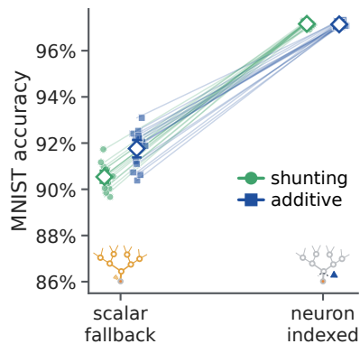
Neuron-indexed feedback
