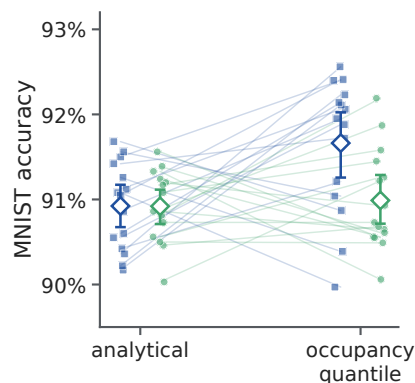
Initialization factorial
