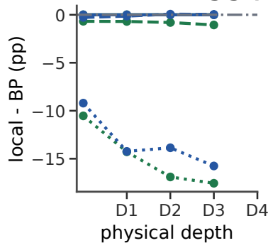
F Local-learning gap
