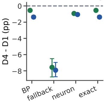
E Fixed-contact depth
