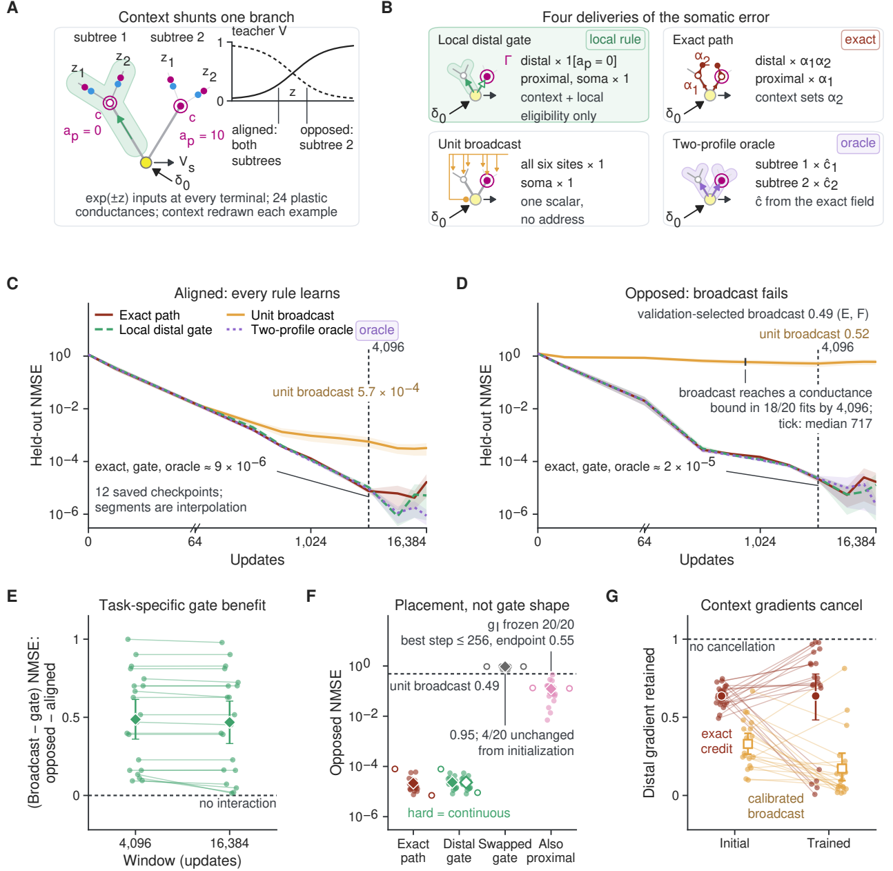
Figure 5: A local inhibitory gate delivers branch-selective credit that matches exact path credit in a conductance tree. A , Seven-compartment circuit: four terminals driven by \exp(\pm z_j) feed two junctions and a soma that \delta_0 enters; binary context raises one junction's inhibitory conductance ( a_p = 10 ; closed, descendants attenuated). Inset, nominal teacher voltage against the latent feature, aligned solid and opposed dashed; fitted teachers are independently perturbed. Blue, excitatory contacts; magenta, inhibitory contacts and the context gate. Schematic, except the inset curves. B , Four deliveries of \delta_0 on identical trees: local distal gate ( \times \mathcal{K}[a_p = 0] at terminals, unit above), exact path ( \alpha factors), unit broadcast and two-profile oracle. The card draws the hard gate; both gates restrict \Gamma (Eq. 4) to \{0, 1\} and (0, 1] and both appear in F . Schematic, no data. C, D , Held-out NMSE for aligned and opposed targets; means of 20 paired seeds with 95% pointwise whole-seed bootstrap bands; rule key in C (exact path solid, local distal gate dashed, two-profile oracle dotted, unit broadcast solid), tick in D at the median first bound contact, 717 updates. Exact path, gate and oracle coincide within the line width from 256 updates. E , Opposed-minus-aligned difference in broadcast-minus-gate NMSE at both windows, hairlines joining seeds; dashed rule, zero interaction; n = 20 paired seeds, 95% paired whole-seed bootstrap intervals at validation-selected states, prespecified sign-flip P = 3.8 \times 10^{-6} (Holm). F , Opposed NMSE within the 4,096-update window by gate shape and placement; filled marks, the hard gate \mathcal{K}[a_p = 0] ; open marks, the continuous gate 1/(1 + g_p^I a_p) ; small open circles, the same condition at Adam 0.01 (left) and 0.1 (right); dashed rule, unit broadcast. At the swapped gate and both gate shapes, spread and intervals are narrower than the markers. n = 20 seeds per condition and rate, 95% whole-seed bootstrap intervals, validation-selected states. G , Earlier cohort: distal gradient retained after context averaging at initial and broadcast-trained weights, hairlines joining each seed across states; dashed rule at 1, no context cancellation. Exact-credit means coincide at the two states but the trained distribution splits, five of twenty seeds below 0.17. n = 20 seeds, 95% whole-seed bootstrap intervals, narrower than the markers at the initial state. Source Data: source_data/curated_publication/figure_05_plotted.csv .
