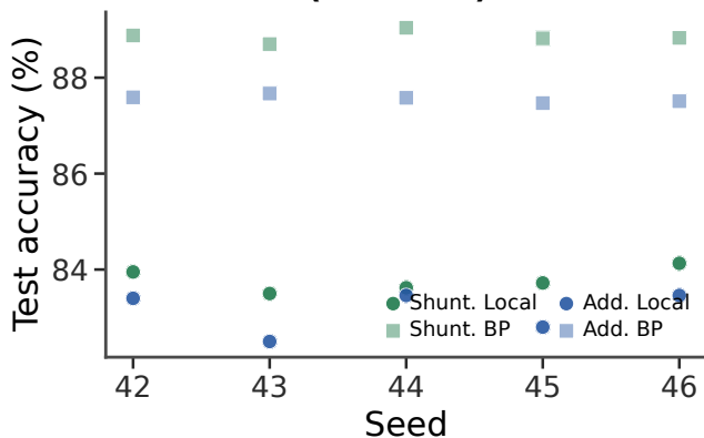
D F-MNIST (all seeds)
