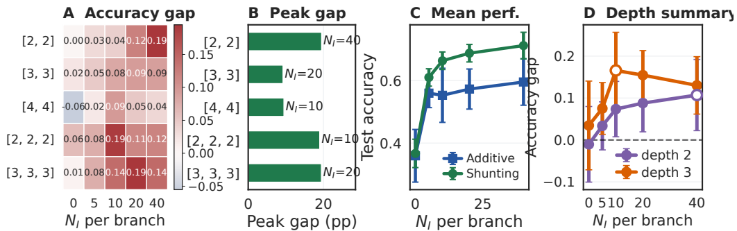
Figure S10: Descriptive morphology \times inhibition performance map. (A) Shunting-minus-additive LocalCA accuracy gap across dendritic morphologies and inhibitory synapse counts. (B) Best inhibitory count for each morphology. (C) Mean performance across tested trees. (D) Average shunting advantage by depth, with markers showing the peak inhibitory count for each depth. The grid uses nonnegative inputs. Because analytical initialization places one shunting population at a near-zero coupling floor, these comparisons are descriptive rather than a causal morphology intervention.
