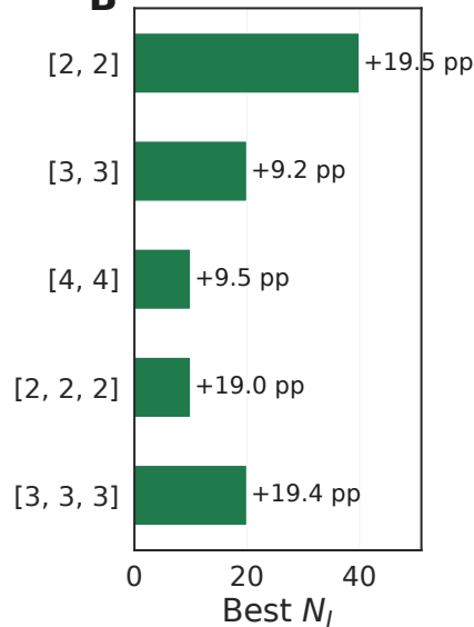
Best inhibition by tre
