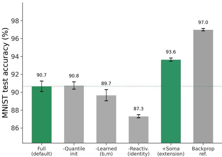
(A) Shunting (MNIST)
