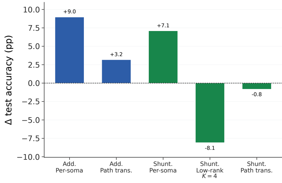
Matched shift from soma-off
