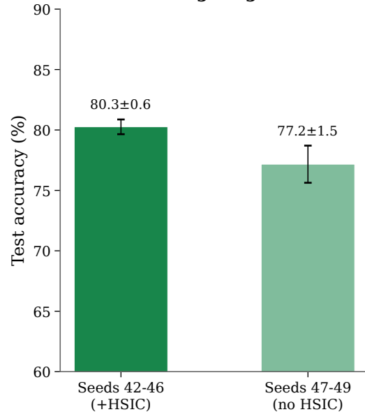
Context gating verif.
