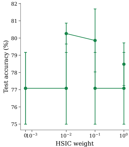
CG: HSIC ablation
