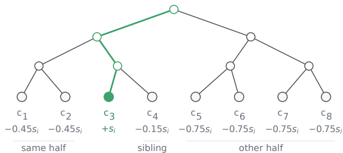
Learning across channel budgets
