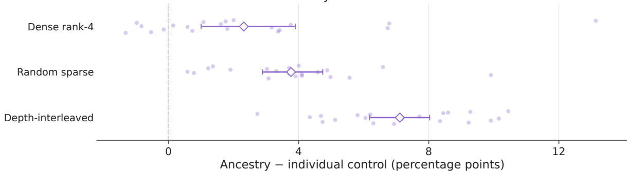
K = 4: ancestry versus individual controls
