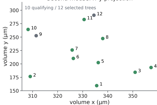
Second mouse: x-y projection
