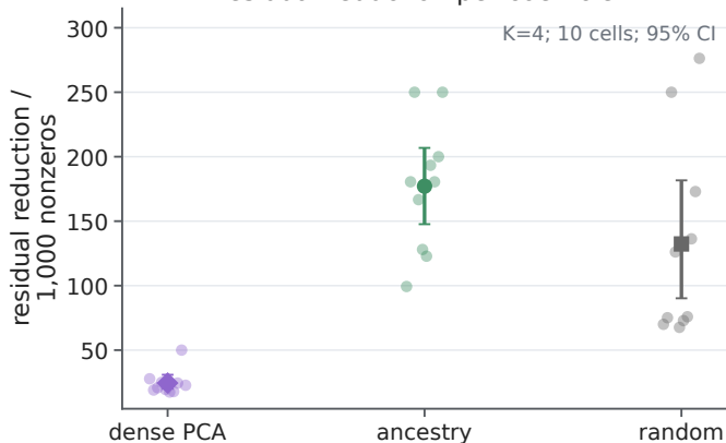
Residual reduction per coefficient
