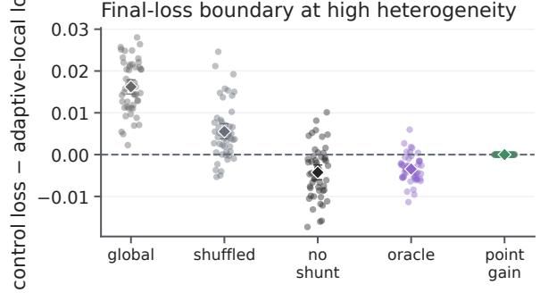
Figure S24: Locally estimated reliability recovers placement ordering but not an absolute shunting advantage. This synthetic positive-rate binary task uses eight parallel, nonserial branch blocks with heterogeneous signal and noise; it is not a reconstructed arbor or a physical-depth experiment. A , Two independent noisy local gradient observations estimate branch signal and noise moments, \hat{S}_b and \hat{N}_b , which set gain a_b and nonnegative shunt \kappa_b for branch b ; c is the fixed step fraction. B , Fixed initial-oracle and final adaptive attenuation profiles at maximum heterogeneity; adaptive points show mean \pm s.d. over 50 independent seeds. C , Final test loss after 40 updates across reliability heterogeneity, comparing adaptive local, global and shuffled gains with no shunt and the fixed initial oracle. Curves and shading are means and 95% seed-bootstrap intervals. D , Control minus adaptive-local final loss at maximum heterogeneity; positive values favor adaptive local. Small points are paired seeds and large symbols are means with 95% paired-seed bootstrap intervals. Adaptive local beats global and shuffled attenuation, loses to no shunt and the fixed initial oracle, and is numerically identical to the independently computed point gain.
