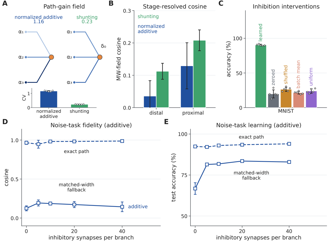
Figure S1: Mechanistic chain from path gains to learning in regular-tree models. MNIST panels A–C use two-stage [4,4] directed trees; the synthetic noise-resilience panels D,E use two-stage [3,3] additive trees. A , Conductance-stage path-gain field in shunting and normalized-additive models at five inhibitory synapses per branch; the inset shows paired-seed coefficients of variation (CV; standard deviation divided by mean). The displayed \alpha values are path gains and \delta_0 is the somatic error. This loading quantity omits branch derivatives and is distinct from the trained exact-error profiles in Supplementary Fig. S45D,E. B , Stage-resolved cosine of matched-width (MW) scalar-fallback versus exact MNIST errors; the width-matched somatic stage is excluded because its cosine is one by construction. C , MNIST post-training inhibition interventions: zero, sample shuffle, per-branch batch mean and a uniform matched mean. These also change forward computation and do not isolate backward shunting. D,E , Feedback fidelity and learning on the additive noise task; solid and dashed lines denote matched-width scalar-fallback and exact transport. Bars show standard deviations across checkpoints in B and retained runs in C–E ; white points in C identify runs. Historical noise-task shunting aggregates with unresolved execution lineage are excluded and retained in Source Data only. The retained additive aggregates do not resolve their normalization setting. The state-matched focal analysis in main Fig. 7 provides the conductance-specific transport comparison.
