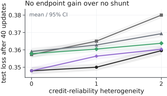
Figure S24: Locally estimated reliability recovers placement ordering but not an absolute shunting advantage. This synthetic positive-rate binary task uses eight parallel, nonserial branch blocks with heterogeneous signal and noise; it is not a reconstructed arbor or a physical-depth experiment. A , Two independent noisy local gradient observations estimate branch signal and noise moments, \hat{S}_b and \hat{N}_b , which set gain a_b and nonnegative shunt \kappa_b for branch b ; c is the fixed step fraction. B , Fixed initial-oracle and final adaptive attenuation profiles at maximum heterogeneity; adaptive points show mean \pm s.d. over 50 independent seeds. C , Final test loss after 40 updates across reliability heterogeneity, comparing adaptive local, global and shuffled gains with no shunt and the fixed initial oracle. Curves and shading are means and 95% seed-bootstrap intervals. D , Control minus adaptive-local final loss at maximum heterogeneity; positive values favor adaptive local. Small points are paired seeds and large symbols are means with 95% paired-seed bootstrap intervals. Adaptive local beats global and shuffled attenuation, loses to no shunt and the fixed initial oracle, and is numerically identical to the independently computed point gain.
