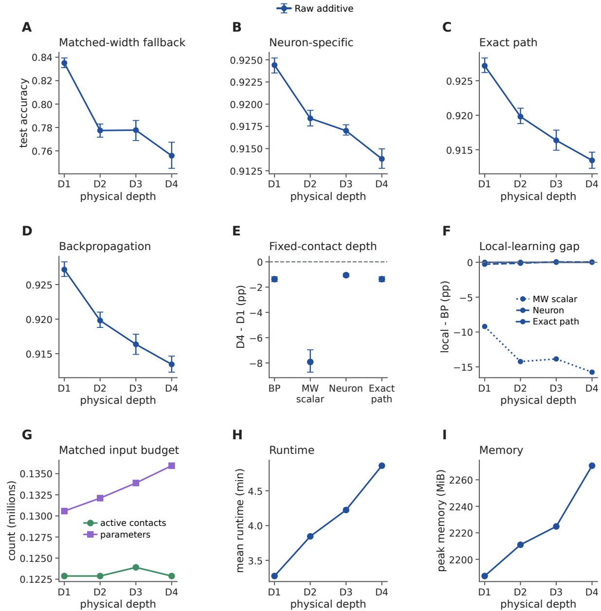
Figure S8: Fixed terminal-branch and input-contact budgets do not make greater dendritic depth intrinsically beneficial. The synthetic noise-resilience task uses conductance-valid raw-additive trees with 16 terminal branches: D1 [16], D2 [4, 4], D3 [2, 2, 4] and D4 [2, 2, 2, 2]. These cohort-specific labels are not the morphologies in Supplementary Fig. S31. The experiment asks whether accuracy rises when fixed terminal and contact budgets are distributed across more serial stages. A–D , Held-out accuracy under matched-width scalar-fallback, neuron-specific, exact-path and backpropagated learning, respectively. E , Prespecified D4-minus-D1 accuracy contrasts, in percentage points (pp). F , Local-minus-backpropagated (BP) accuracy in pp; line styles identify the three local fields. G , Active contacts and trainable parameters. H, I , Runtime in minutes and peak memory in mebibytes (MiB). Each condition has ten paired seeds; symbols and intervals are means and 95% paired-seed bootstrap intervals. All four retained D4-minus-D1 contrasts were negative in 10/10 pairs (Wilcoxon P = 0.001953 ). The design fixes 16 terminals and 960–968 active contacts per soma, but not compartment or parameter count. Shunting series fail the nonnegative-conductance criterion on this task and are excluded from inference.
