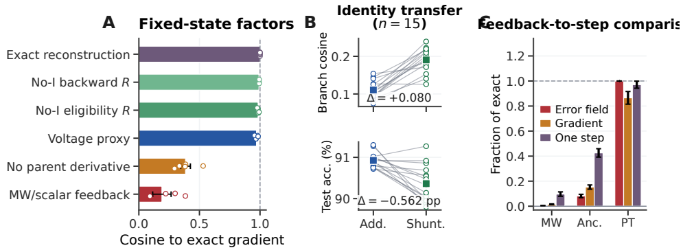
Figure S3: Mechanistic analysis separating path effects from learning consequences. (A) Fixed-forward-state factor substitutions in five shunting checkpoints. Removing inhibitory conductance from either resistance factor leaves gradient direction close to exact reconstruction, whereas omitting parent transfer derivatives or using matched-width/scalar-fallback feedback causes larger directional errors. Bars are mean \pm s.e.m.; points are seeds. (B) Fifteen paired identity-transfer checkpoints. Shunting improves branch-gradient direction, while additive test accuracy remains slightly higher; squares denote means. (C) The same-batch feedback ladder measured as optimally rescaled dendritic error-field capture, eligibility-weighted branch-gradient capture, and norm-matched one-step progress at relative step 10^{-5} . Bars pool five checkpoints per core after averaging three diagnostic splits; error bars are s.e.m. over checkpoints. In this cohort the global scalar equals the matched-width/scalar-fallback field, and the available ancestry field equals exact-soma ancestry. Error geometry alone is therefore not treated as a learning metric. Fixed-state substitutions are diagnostic hybrids, not separately trained forward models.
