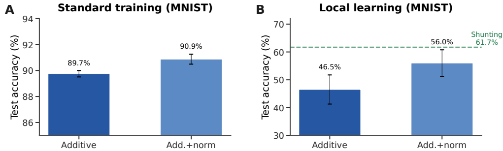
Figure S9: Additive + normalization control (MNIST stress-regime diagnostic). (A) Standard backprop: normalization provides a small boost (89.7% \rightarrow 90.9%). (B) Local learning: normalization improves additive from 46.5% to 56.0% (+9.5 pp), partially closing the gap to shunting (61.7%, dashed green). These lower local accuracies come from a separate stress-regime diagnostic, not from the matched-capacity performance setting in Table S8.
