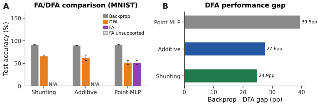
Figure S7: Feedback alignment baselines (MNIST) . (A) Grouped comparison: standard backprop (neutral gray), DFA (orange), and FA (purple). Hatched N/A markers indicate that FA is not implemented for the block-structured dendritic architectures because the random feedback matrices are not dimensionally compatible with the tree-structured branch updates. DFA achieves 66.1% on shunting vs. 62.2% additive vs. 51.8% point MLP. (B) Backprop–DFA gap: dendritic architectures (24.9–27.6 pp) show smaller gaps than point MLPs (39.5 pp), suggesting conductance-based architecture is partially compatible with random feedback.
