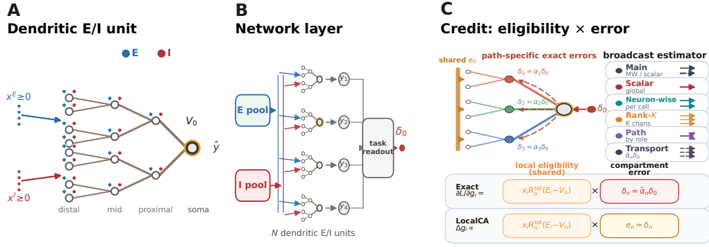
Figure 1: Model and credit assignment. (A) Schematic of a dendritic unit with excitatory and inhibitory inputs on each branch. (B) Layer of such units projecting to a task readout; \delta_0 = \partial L / \partial V_0 is the soma/core error used for feedback. (C) Exact updates multiply local eligibility by path-specific errors \delta_{u,n} ; LocalCA replaces them with broadcast estimates e_{u,n} . The main matched-width/scalar-fallback hybrid is shown separately from strict scalar, neuron-wise, low-rank, path-structured, and transported feedback.
