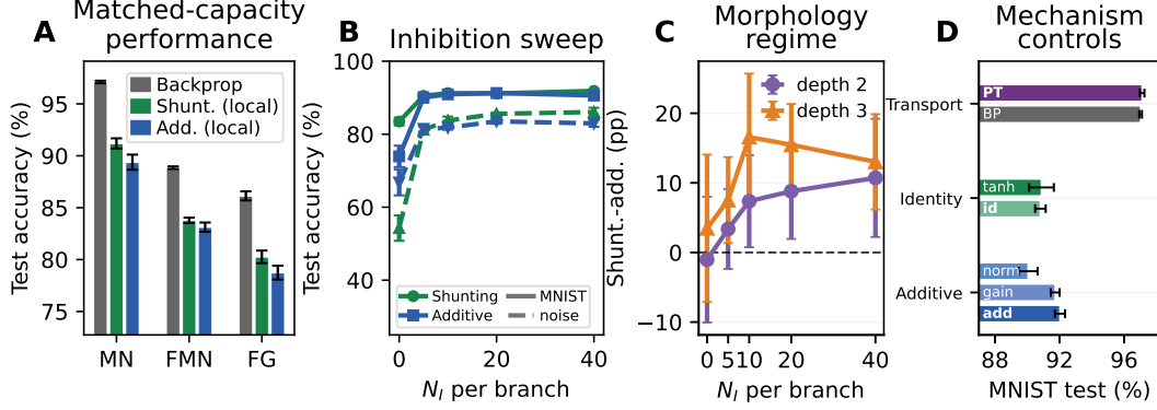
Figure 4: Matched-capacity performance and regime dependence. (A) Matched shunting back-propagation reference vs. per-soma 5F LocalCA; additive backpropagation references are reported in Table S3 where matched five-seed runs are available. (B) Inhibitory dose-response. (C) Morphology-dependent shunting advantage. (D) MNIST controls: BP, exact path transport (PT), activation choice, and additive gain/normalization variants. Values/protocols: Table S3; Appendix A. Error bars denote \pm 1 s.d.
