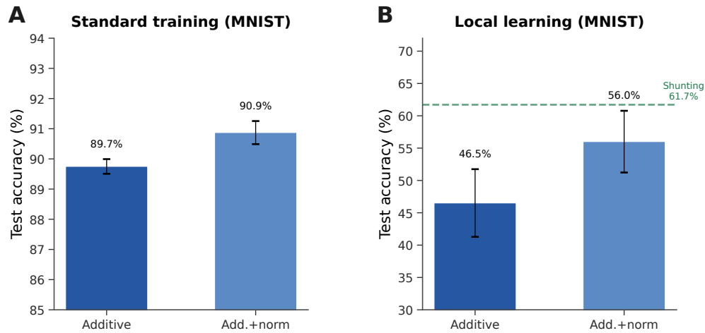
Figure S9: Additive + normalization control (MNIST stress-regime diagnostic). (A) Standard backprop: normalization provides a small boost (89.7% → 90.9%). (B) Local learning: normalization improves additive from 46.5% to 56.0% (+9.5 pp), partially closing the gap to shunting (61.7%, dashed green). These lower local accuracies come from a separate stress-regime diagnostic, not from the capacity-calibrated competence setting in Table S5.
