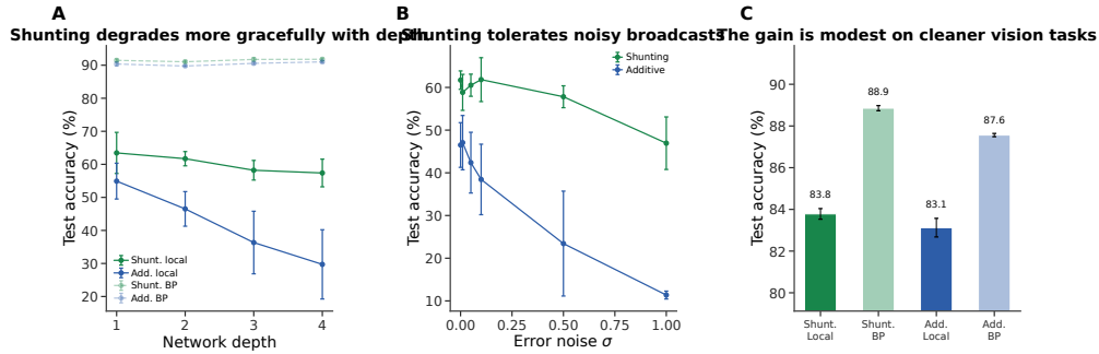
Figure S6: Additional stress tests. (A) Depth scaling: shunting local (green) degrades more gracefully from 63.5\% to 57.4\% ; additive local (blue) drops from 54.9\% to 29.7\% . Backprop ceilings (dashed) remain stable. (B) Broadcast-noise robustness: shunting remains stable for \sigma \leq 0.1 ; additive degrades rapidly and reaches chance at \sigma = 1 . (C) Fashion-MNIST: the shunting gain is modest on this cleaner benchmark ( 83.8\% local vs. 88.9\% backprop), consistent with the regime-dependent story in the main text.
