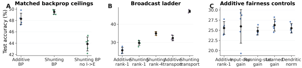
Figure S8: CIFAR-10 control ladder in the compact direct-I-stream family . (A) Matched backprop ceilings. With nonnegative inputs and a nonlinear decoder, shunting slightly exceeds additive under standard training, and removing learned I-to-E conductance lowers the shunting ceiling. (B) Broadcast ladder. Rank-1 broadcast remains weak on this harder dataset, rank-4 improves partially, and exact effective transported error nearly reaches the shunting backprop ceiling. (C) Additive fairness controls. Input-dependent gain, running-stat gain, learned gain, and dendritic normalization do not rescue additive rank-1 broadcast. This figure is a harder-data diagnostic, not a claim of competitive CIFAR-10 benchmarking.
