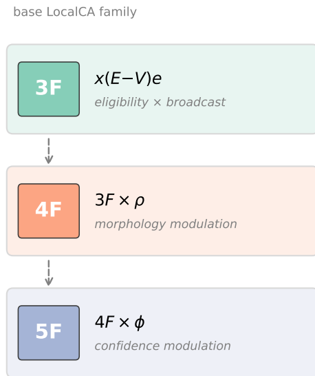
(B) Local learning rule hierarchy
