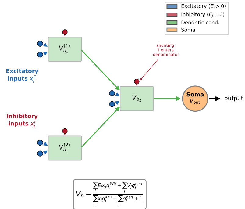
(A) Compartmental dendritic neuron
