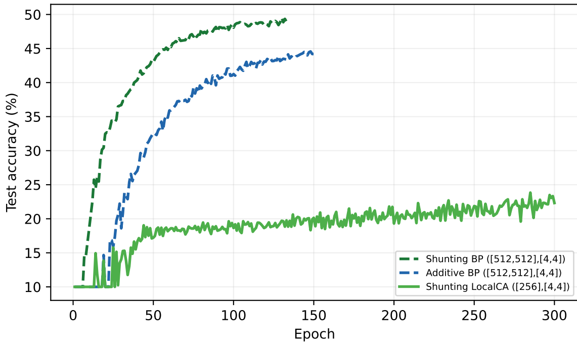
Representative CIFAR-10 Accuracy Curves
