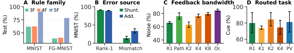
Figure 5: Rule and feedback controls. (A) Eligibility-rule ablation: 3F and 4F learn weakly, while the 5F reliability preconditioner is the practical LocalCA rule used in the competence results. (B) Error-source ablation: soma-derived feedback is essential, whereas local-mismatch feedback is not a usable substitute. (C) Feedback-bandwidth ladder on noise resilience: per-soma feedback, path-propagation, random low-rank feedback, and [C] exact transported error form a monotonic fidelity ladder. (D) Cue-routing feedback-rank diagnostic: richer feedback helps relative to the restricted baseline, while pathway-vector feedback remains an exploratory structured control.
