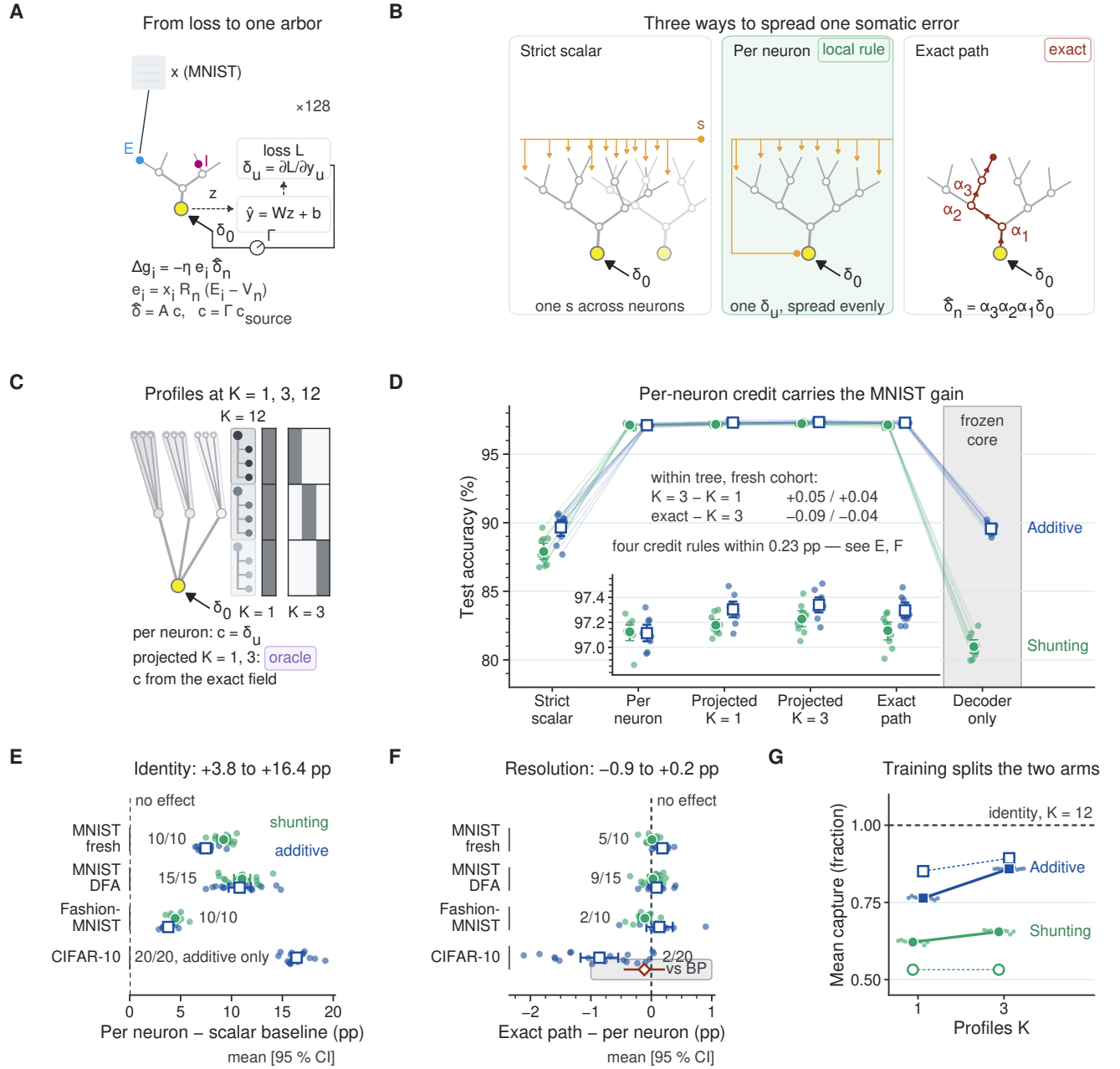
Figure 1: Neuronal identity, not finer spatial address, carries the image-learning benefit. A , MNIST input (leader) reaches an excitatory contact (blue) on one of 128 trees; an inhibitory contact (carmine) is also drawn. The arbor is schematic, not C's [3, 3] morphology. Readout \hat{y} and loss \mathcal{L} return \delta_u into the soma as \delta_0 (ink arrow) through the diagonal gain \Gamma (dial), c = \Gamma c_{\text{source}} ; no data. B , Three deliveries on a generic depth-three tree: a strict scalar s shared with a ghosted neighbour, one signal per neuron, and the exact path \hat{\delta}_n = \alpha_3 \alpha_2 \alpha_1 \delta_0 ; schematic, no data. C , Dictionaries over the twelve nonsomatic sites: the tinted strip is the K = 12 identity, beside K = 1 all-ones and K = 3 proximal subtrees; columns are indicator supports averaged by the projected rules (oracle badge); schematic, no data. D , Test accuracy for six rules at selected rates; circles shunting, squares additive, dots seeds paired by hairlines; band, decoder only; note, the fresh-cohort within-tree contrasts; means with 95% seed-bootstrap intervals over ten fresh paired seeds per architecture, smaller than the symbol for per neuron, projected K = 1, 3 and exact path. Inset, those four columns at the same x positions and marks, rescaled until their intervals and ten seeds resolve. E , Per neuron minus each cohort's scalar baseline (the strict scalar, except the matched-width fallback for Fashion-MNIST), shunting on the row and additive open below it, except additive-only CIFAR-10, drawn on its row; each row tagged with the on-row arm's positive seeds out of the total ( n = 10, 15, 10 and 20 seeds); means with paired 95% seed-bootstrap intervals (Student- t for CIFAR-10) in percentage points, several narrower than the symbol. F , Exact path minus per neuron in the same rows, marks and interval type; in the CIFAR-10 row the open red-brown diamond and interval are exact path minus backpropagation, inside the band of the prespecified \pm 1 percentage-point margin. G , Mean activation-error capture of D 's exact-path fields by C 's dictionaries at K = 1, 3 ; filled, trained state, with its ten seeds; open, initialization ( n = 10 , seeds not drawn); reference line at 1, the K = 12 identity, which reproduces the field. All 95% seed-bootstrap intervals are at most 0.007 capture units and are not drawn. pp, percentage points. Source Data: source_data/curated_publication/figure_01_plotted.csv .
