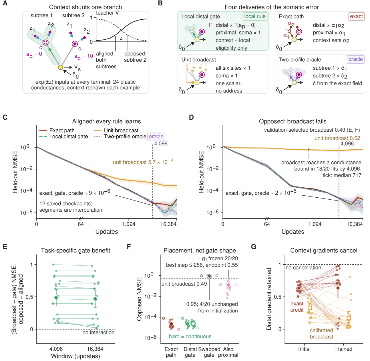
Figure 5: A local inhibitory gate delivers branch-selective credit that matches exact path credit in a conductance tree. A , Seven-compartment circuit: four terminals feed two junctions and a soma that \delta_0 enters; binary context raises one junction's inhibitory conductance ( a_p = 10 , closed, descendants attenuated). Inset, the nominal unperturbed teacher terminal voltage, increasing solid and decreasing dashed; fits used independently perturbed teachers. Blue, excitatory contacts; magenta, inhibitory contacts and the context gate; green, the local gate's target subtree. Schematic, except the inset. B , Four deliveries of \delta_0 on identical trees: local distal gate ( \propto \mathcal{K}[a_p = 0] at terminals, unit above), exact path ( \alpha factors), unit broadcast and two-profile oracle. The local gate's card draws the hard form, restricting \Gamma (Eq. 4) to \{0, 1\} ; its continuous form in F gives (0, 1] . Schematic. C, D , Held-out NMSE for aligned and opposed targets; means of 20 paired seeds with 95% pointwise bootstrap bands; rule key in C (exact path solid, gate dashed, oracle dotted, unit broadcast solid); tick in D , the median first bound contact at 717 updates. Exact path, gate and oracle coincide within the line width from 256 updates to the 4,096-update rule, and separate beyond it. E , Opposed-minus-aligned difference in broadcast-minus-gate NMSE at both windows, hairlines joining seeds; dashed rule, no interaction; n = 20 paired seeds, 95% paired whole-seed bootstrap intervals at validation-selected states, sign-flip P = 3.8 \times 10^{-6} (Holm). F , Opposed NMSE in the 4,096-update window by gate shape and placement; at the distal-gate tick the filled and open diamonds are the hard gate \mathcal{K}[a_p = 0] and the continuous gate 1/(1 + g_p^l a_p) , both with filled seed clouds; small open circles, each column's rule at Adam 0.01 (left) and 0.1 (right); dashed rule, unit broadcast. At the swapped gate, spread and intervals are narrower than the markers; at the two shapes only the intervals are. n = 20 seeds per condition and rate, 95% whole-seed bootstrap intervals, validation-selected states. G , Earlier cohort: distal gradient retained after context averaging at initial and broadcast-trained weights, hairlines joining seeds; dashed rule at 1. Exact-credit means coincide at the two states but the trained distribution splits, five of twenty below 0.17. n = 20 seeds, 95% whole-seed bootstrap intervals. Source Data: source_data/curated_publication/figure_05_plotted.csv.
