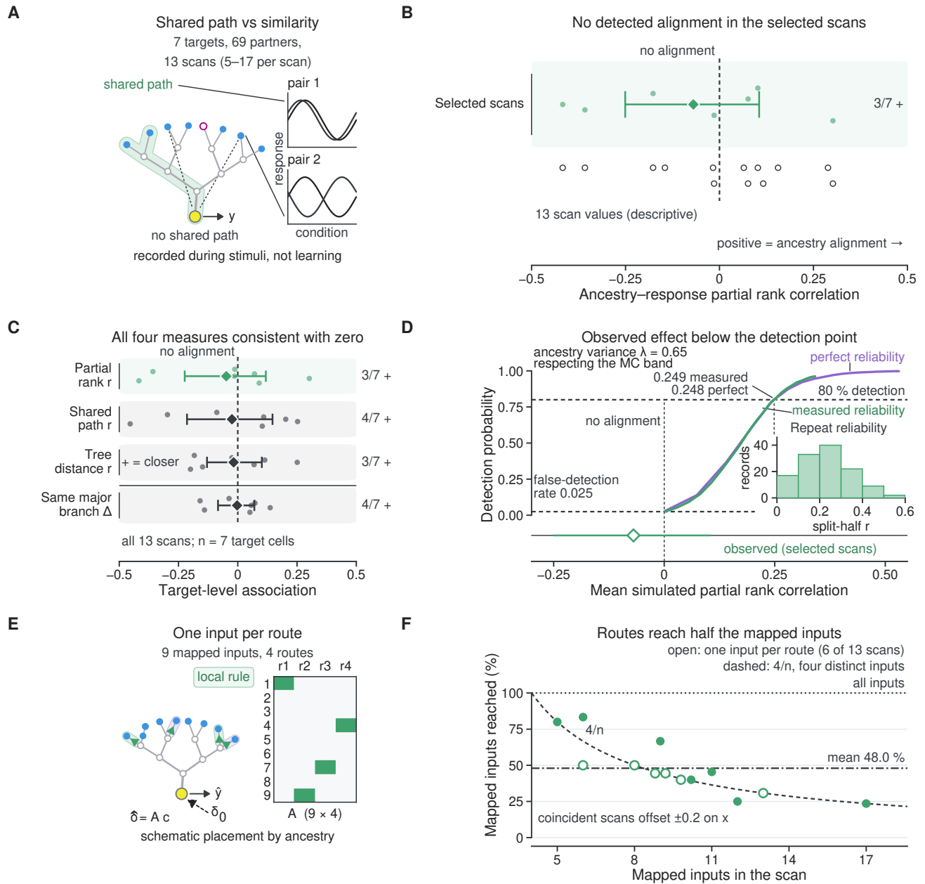
Figure 9: Recorded partner responses show no detected dendritic-ancestry alignment, and this sample reaches 80% detection only above a partial rank correlation of about 0.25. A , Two contact pairs on one arbor, one sharing a soma-to-ancestor path (green patch), the other linked to the soma by dashed hairlines; filled blue discs, excitatory contacts; open magenta ring, an inhibitory partner; right, their responses. No data: stimulus recordings, no \delta_0 . B , Ancestry–response partial rank correlation, selected scans; dots, the seven target values; open circles, the thirteen all-eligible-scan values (same targets, stacked where they would overlap); diamond, mean with 95% target-bootstrap interval ( n = 7 ): -0.069 [-0.251, 0.106] ; right, 3/7 +, targets with positive values. C , Same inference, four topology measures, all thirteen scans ( n = 7 ; 95% target-bootstrap intervals). Top row, the all-eligible-scan partial rank correlation, -0.048 [-0.224, 0.118] . Tree distance is sign-flipped. Below the rule, same-major-branch \Delta is a difference in mean similarity, not a correlation; its narrower interval reflects that smaller scale, not greater precision. D , Detection probability against the frozen model’s mean simulated partial rank correlation; shaded 95% Wilson Monte Carlo intervals (half-width \leq 0.016 , narrower than the stroke); intercepts, false-detection rates: 0.025 measured, 0.030 perfect. Open diamond and bar below the axis, the observed estimate ( n = 7 , 95% target bootstrap), not power. Inset, split-half repeat reliability, 125 partner–scan records from 102 partners; 123 drawn, the two with negative r omitted. E , Representative scan (median mapped-input count, not outcome-selected): nine mapped inputs beside the realized 9 \times 4 support, \hat{\delta} = A c imposed, not observed (schematic; dashed \delta_0 ). Route-capsule tints and the local rule badge covering the card encode no per-route property. F , Mapped inputs reached per scan; open, the six scans whose four routes each reached one input; dashed, 4/n, coverage when four routes reach distinct inputs. Not a ceiling: two scans fall below (repeated inputs), three above (multi-input routes). Coincident scans are offset \pm 0.2 ; n = 13 scans from seven targets, descriptive. Source Data: source_data/curated_publication/figure_09_plotted.csv , source_data/functional_topology_all_scans/ , source_data/credit_first_figures/ (figure_08_sources.json, figure_08_support.csv and figure_08_actual_support.npz).
