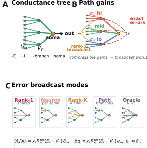
Figure 1: Model and credit assignment. (A) Conductance tree with nonnegative excitatory drive and inhibitory shunting load. (B) Exact credit is path-specific, whereas rank-1 LocalCA broadcasts one shared error field. (C) LocalCA keeps the exact synapse-local eligibility and substitutes e_n \approx \delta_n ; rank-1, neuron-wise, rank- K , and path-structured broadcasts trade biological bandwidth for fidelity, while transported error is an oracle.
