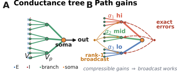
Figure 1: Model and credit assignment. (A) Conductance tree with nonnegative excitatory drive and inhibitory shunting load. (B) Exact credit is path-specific, whereas rank-1 LocalCA broadcasts one shared error field. (C) LocalCA keeps the exact synapse-local eligibility and substitutes e_n \approx \delta_n ; rank-1, neuron-wise, rank- K , and path-structured broadcasts trade biological bandwidth for fidelity, while transported error is an oracle.
