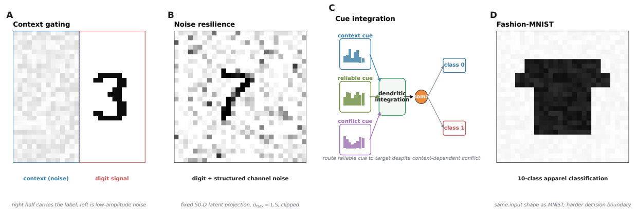
Figure S23: Synthetic benchmark schematics. (A) Context gating: the right half carries the MNIST digit; the left half is filled with low-amplitude uniform noise. (B) Noise resilience: MNIST image corrupted by structured channel noise (fixed 50-D latent projection, \sigma_{\text{task}} = 1.5 , clipped to [0, 1] ). (C) Cue integration: a context cue selects which of two noisy cue streams is reliable; dendritic integration routes the reliable cue to the binary readout. (D) Fashion-MNIST: 10-class apparel classification sharing the MNIST input shape.
