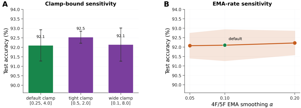
Figure S4: 5F sensitivity analysis (MNIST, shunting, per-soma broadcast). (A) Sensitivity to the \phi_n clamp interval. The default clamp [0.25, 4.0] is already strong ( 92.1 \pm 0.8\% ); tightening it to [0.5, 2.0] slightly improves performance ( 92.5 \pm 0.3\% ), while widening it to [0.1, 8.0] is effectively neutral ( 92.1 \pm 0.9\% ). (B) Sensitivity to the 4F/5F EMA rate used for online statistics. Varying \alpha from 0.05 to 0.20 changes mean test accuracy by less than 0.2 pp. Together these results suggest that the 5F gain is not driven by a brittle single hyperparameter choice, even though the factor itself remains heuristic. Errors: \pm 1 s.d. across 3 seeds.
