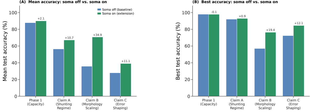
Figure S16: Soma-on extension for LocalCA. Enabling direct somatic input ( somatic_synapses=true ) improves aggregate mean test accuracy across all four manuscript LocalCA families. Each family is summarized over the completed configurations in matched soma-off and soma-on sweeps. The largest gain appears in morphology scaling, where the family mean rises from 35.8% to 70.7% and the best run rises from 57.0% to 76.4%. Gains in the shunting-regime and error-shaping families are smaller but still substantial. Delta labels show soma-on minus soma-off. Because the main mechanistic analysis was developed in the dendrite-only feedforward regime, we report soma-on as a supportive extension rather than replacing the main operating regime.
