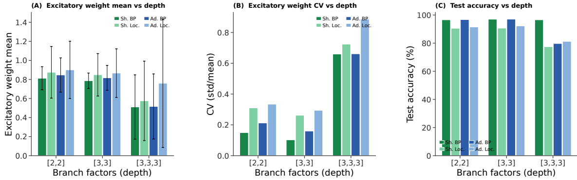
Figure S21: Synaptic weight statistics vs. dendritic depth (MNIST, 5 seeds/cell). (A) Excitatory weight mean (error bars = std). At [2,2] and [3,3], all four conditions cluster around 0.8–0.9; at [3,3,3] the means drop to \approx 0.5 –0.75 and the cross-seed spread grows, especially for additive LocalCA. (B) Coefficient of variation (CV = std/mean). At shallow/medium depth, LocalCA produces \sim 2\times higher CV than matched BP, but both remain well-behaved ( \leq 0.33 ). At the deepest network all four conditions jump to CV \approx 0.66 –0.88, with additive LocalCA the broadest. (C) MNIST test accuracy. BP tracks \sim 96 –97% at [2,2]/[3,3] and \sim 92 –95% at [3,3,3]. LocalCA stays within \sim 5 –6 pp of BP at shallow/medium depth but trails by \sim 15 –20 pp at [3,3,3], identifying depth as the remaining open challenge for this local rule. The qualitative ordering (shunting LocalCA tracks shunting BP more closely than additive LocalCA tracks additive BP) reinforces the manuscript claim that the conductance denominator is the key mechanistic ingredient.
