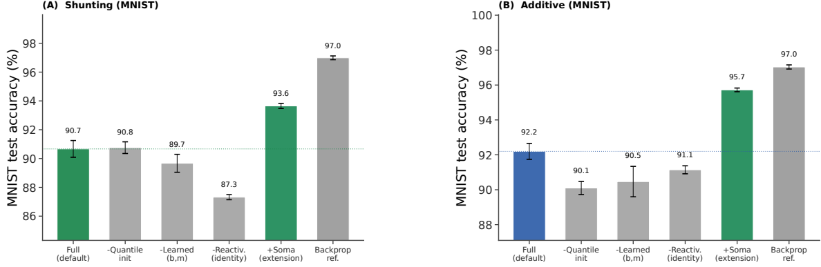
Figure S19: Per-component ablation for LocalCA on MNIST. Bars show mean test accuracy ( \pm s.d. across 5 seeds); coloured bars highlight the manuscript default (blue/green) and the soma-on extension (green). (A) Shunting: The full default reaches 90.7%; removing quantile init leaves accuracy unchanged at 90.8% (quantile init is a mild calibration nudge on this clean task), removing learned ( b, m ) drops by about 1 pp, and removing reactivation entirely drops accuracy to 87.3%; the reactivation transform is the largest single LocalCA ingredient. (B) Additive: Quantile init contributes +2.1 pp (90.1 \rightarrow 92.2%), learned ( b, m ) contributes +1.7 pp, and reactivation contributes +1.1 pp; each ingredient helps on the additive core. Soma-on is the largest positive change in both cores (+3 to +3.5 pp over full config), while matched standard backpropagation reaches 97.0% in both cores and sets the upper reference. The fixed-relu reactivation condition did not satisfy the same initialization checks and is omitted.
