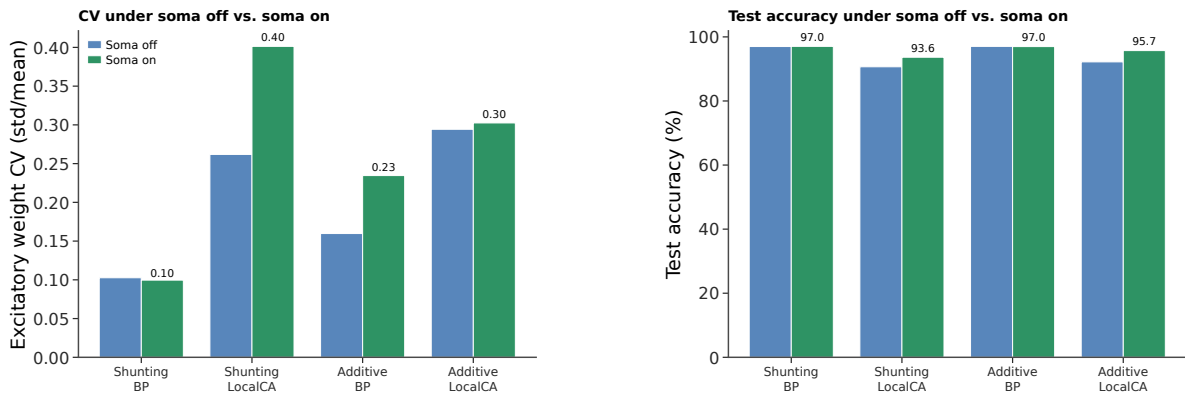
Figure S22: Excitatory-weight CV and MNIST accuracy under soma-off vs. soma-on (depth [3,3], 5 seeds/cell). (A) Coefficient of variation of excitatory weights for the four (core, strategy) cells; paired bars show soma-off (from Fig. S21) and soma-on (this sweep). Shunting + BP tightens slightly; shunting + LocalCA broadens; additive cells change little. (B) Matched MNIST test accuracy (sanity panel). BP accuracy is preserved or marginally improved; LocalCA accuracy is preserved for additive but drops \sim 3 pp for shunting, consistent with the CV widening in panel A.
