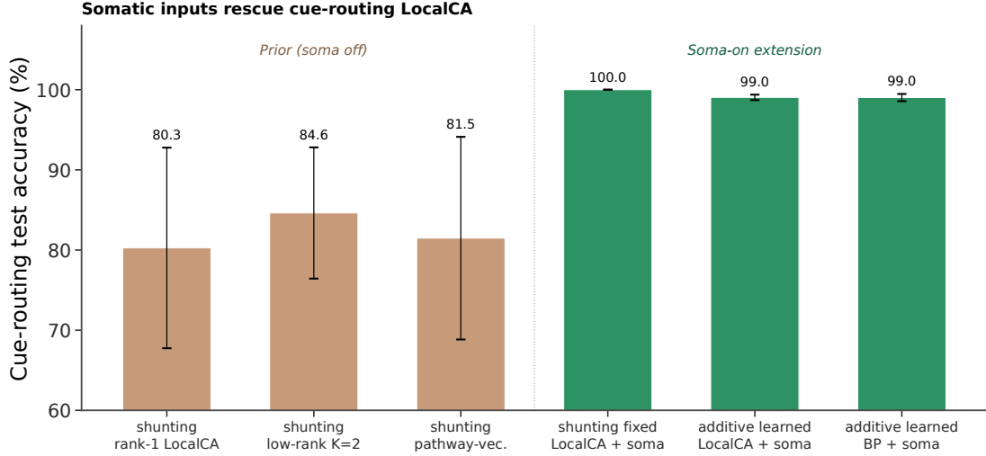
Figure S17: Soma-on rescues cue-routing LocalCA. The left bars show the previously reported soma-off LocalCA results on the cue-integration benchmark. The right bars show the soma-on extension: fixed-router shunting LocalCA reaches 1.00 test accuracy, and learned-router additive LocalCA with soma reaches 0.99, matching the additive backprop ceiling with soma. The soma channel supplies a direct high-bandwidth input that bypasses the rank-1 bottleneck identified in the main text. Learned-router shunting with soma is omitted because this benchmark uses signed cues, which conflict with the shunting positive-input check in the learned-router pipeline; fixed-router shunting is therefore the clean shunting data point.
