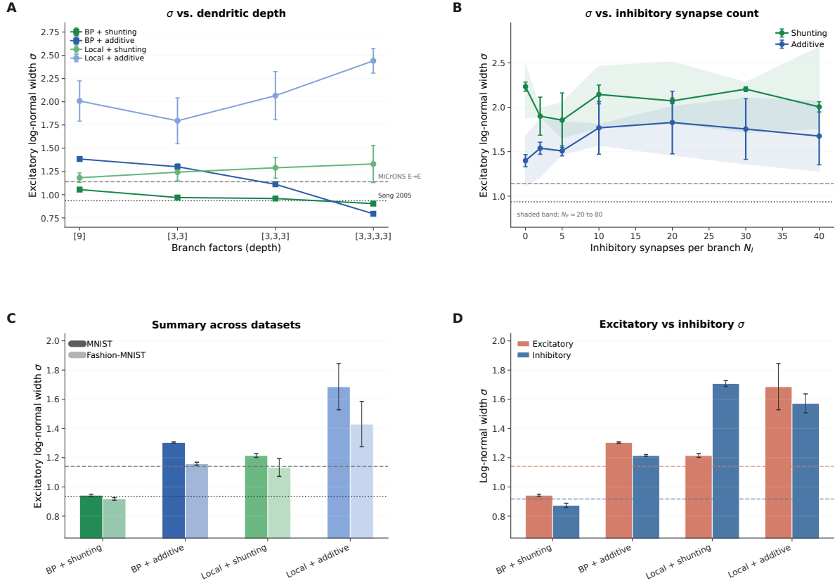
Figure S20: Synaptic weight distribution sensitivity to architecture. (A) Log-normal \sigma vs. dendritic depth (branch factors [9] to [3,3,3,3]). Both backprop and local shunting remain closer to the biological-width references than their additive counterparts across depth. (B) \sigma vs. inhibitory synapses per branch ( N_I ). Without inhibition ( N_I=0 ), all conditions are overly broad; with biologically constrained N_I=10-20 , shunting enters the biological range. Shaded bands show the sweep over N_E=20 to 80. (C) Summary of MNIST and Fashion-MNIST results with biological references. The shunting ordering is consistent across datasets. (D) Excitatory vs. inhibitory weight \sigma on MNIST with MICrONS E→E and I→E reference bands.
