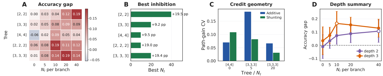
Figure 5: Morphology shifts the useful inhibitory regime. (A) Shunting-minus-additive LocalCA accuracy gap across dendritic morphologies and inhibitory synapse counts. (B) Best inhibitory count for each morphology. (C) Representative path-gain diagnostic for selected morphology cells, used to connect the performance map to credit geometry. (D) Average shunting advantage by depth, with markers showing the peak inhibitory count for each depth.
