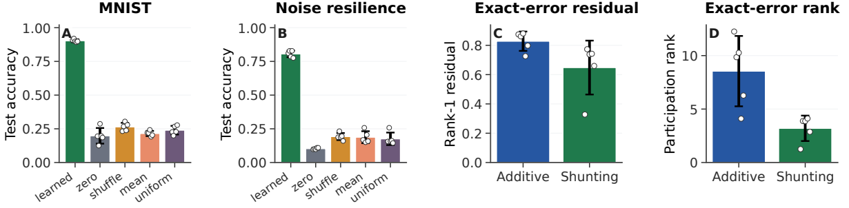
Figure S14: Causal inhibition and exact-error compressibility. (A,B) Post-training inhibitory-conductance interventions on trained shunting LocalCA checkpoints. Accuracy is measured on a 512-example held-out subset; dots show seeds. Removing, shuffling, or clamping learned inhibition collapses performance, showing that the learned inhibitory field carries sample-specific task structure. (C,D) SVD diagnostics of the exact compartment-error matrix on matched MNIST N_I=5 runs. Shunting has a smaller rank-1 residual and lower participation rank than additive, so the exact error field is more compressible. Error bars are s.d. across 5 seeds.
