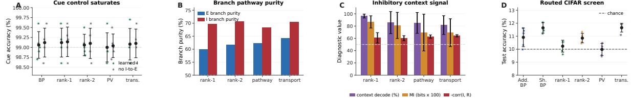
Figure S13: Positive routed-task pathway and inhibition controls. (A) Strictly nonnegative cue-routing controls saturate near 99% for learned-I and no-I variants, so this rerun is not a performance separation. (B) Fitted excitatory and inhibitory synapse banks retain branch-pathway structure above the 50% chance level. (C) In learned-I cue models, pathway-inhibition balance carries context information and inhibitory conductance is negatively coupled to local input resistance. (D) A nonnegative Double-CIFAR contextual screen remains near chance even under matched backprop, so it is not used as evidence for the paper’s local-learning claims. Error bars show s.d. across 5 seeds.
