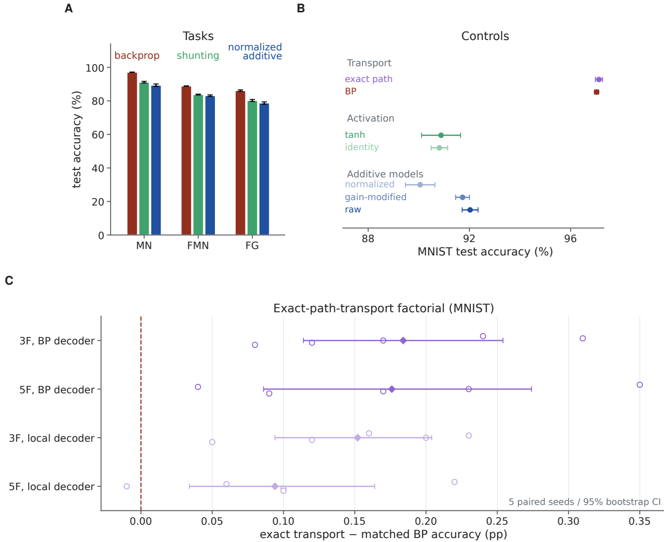
Figure S2: Local eligibility and exact transport reproduce the learning gradient. A , Matched shunting backpropagation and local learning on MNIST, Fashion-MNIST and figure-ground MNIST; blue denotes normalized-additive learning. B , Transport, activation and additive-model implementation controls on MNIST. C , Exact-transport-minus-backpropagation accuracy across three-/five-factor and local/backpropagated decoder choices; points are five paired seeds and bars are 95% paired-seed bootstrap intervals. Exact transport supplies an oracle compartment error. The local three-factor eligibility is sufficient when this error is supplied. Normalized- and raw-additive models are distinct controls; no noise-task shunting aggregate is used here.
