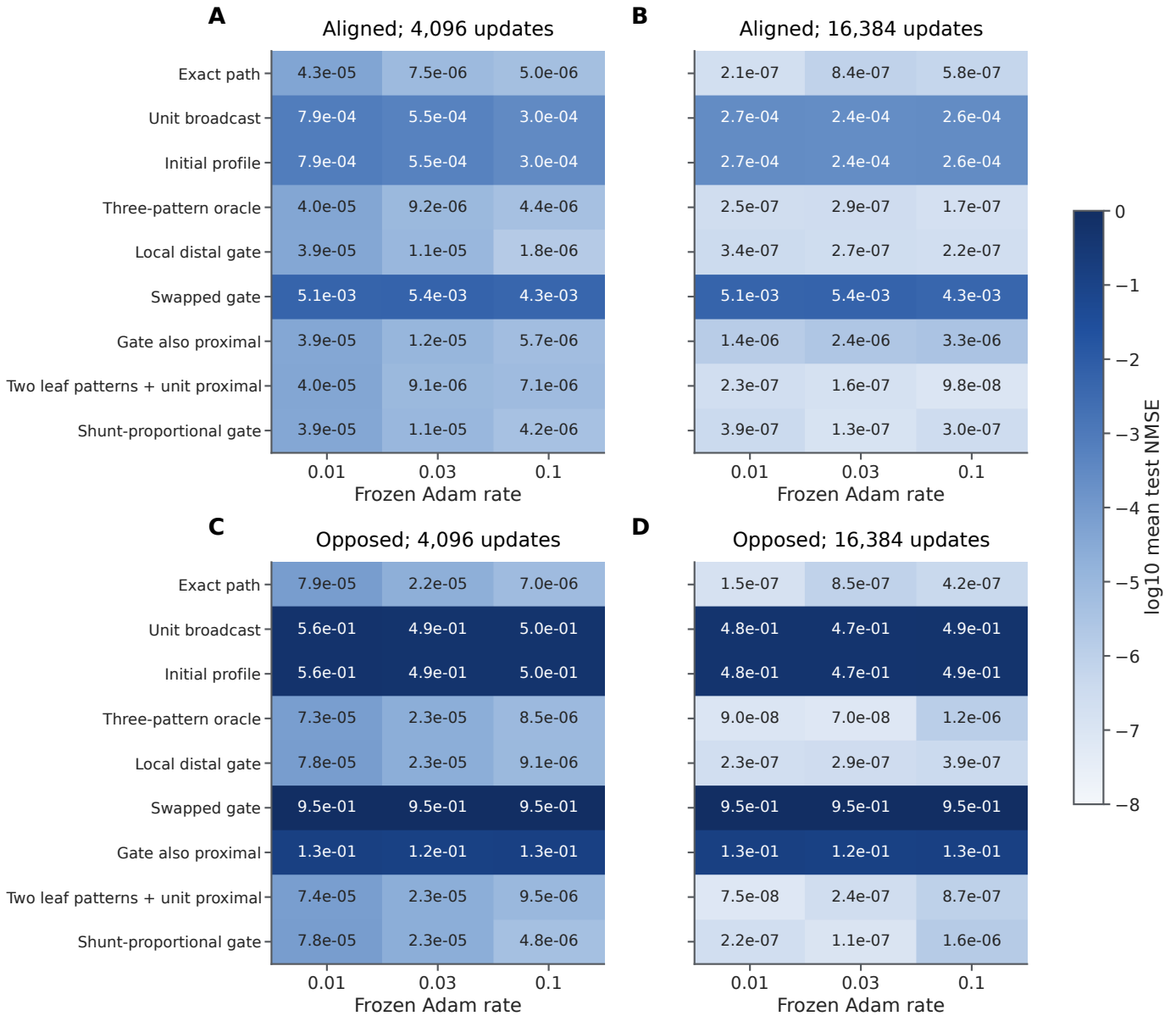
Figure S21: Local conductance gating is robust to rate choice but depends on where it is applied. A,B , Aligned tuning at 4,096 and 16,384 updates. C,D , Opposed tuning at the same budgets. Every rule receives every displayed Adam rate; 0.03 is primary. Entries are mean test NMSE at validation-selected checkpoints across twenty new paired seeds; the color scale shows base-ten logarithm. Unit and calibrated broadcast agree to two significant figures in every cell and are read as one broadcast row. Exact credit, the three-pattern oracle, the local distal gate and the shunt-proportional gate learn accurately. Swapping the gate fails; extending the gate to proximal compartments leaves a substantial opposed-task deficit. The two leaf patterns with unit proximal feedback isolate this placement effect. These are supplied-context, bounded-conductance experiments; the local gate does not estimate arbitrary route coefficients. Both budgets and all rates and seeds remain included; the historical cancellation cohort of the same study is drawn at the main-text type scale in main Fig. 5G.
