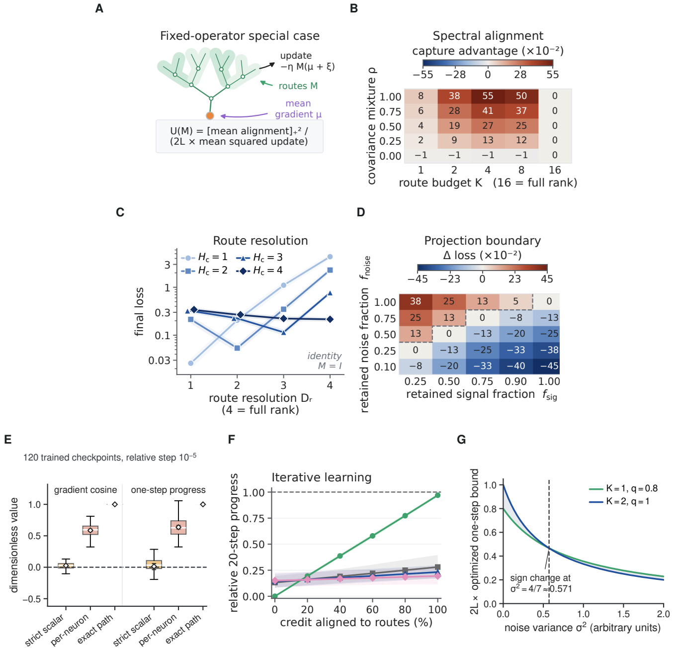
Figure S3: Restricted routes trade signal retention against admitted noise, and the one-step quantity is measurable at trained states. A , Fixed-operator version of the one-step utility bound: the delivered update is M(\mu + \xi) , with mean gradient \mu and zero-mean noise \xi . B , Subtree-minus-random capture across route budget and covariance-mixture coefficient; only the endpoints are isospectral. C , Final quadratic loss when the signal hierarchy and amplified fine-scale noise make an interior route resolution favorable by construction. D , Exact one-step projection boundary: retaining signal fraction f_{\text{sig}} and noise fraction f_{\text{noise}} changes normalized loss by (f_{\text{noise}} - f_{\text{sig}})/2 . E , Candidate/exact gradient cosine and norm-matched one-step loss decrease at the same 120 valid trained checkpoints, drawn on one dimensionless axis; boxes summarize checkpoints and diamonds with bars are means and 95% checkpoint-bootstrap intervals from a single held-out batch at relative step 10^{-5} . F , A separate constructed positive control on eight reconstructed arbors: loss reduction after twenty projected steps against the full-gradient sequence. Green denotes morphology-selected routes, gray random paths, blue depth bins and pink ancestry-shuffled routes; symbols are cell means with hierarchical 95% bootstrap intervals. G , Illustrative rank-noise trade-off under isotropic noise: twice the smoothness constant L times the optimized one-step bound is q^2/(q + K\sigma^2) , comparing (K, q) = (1, 0.8) and (2, 1) , with the sign change shaded; analytic, no data, and not an endpoint-selection prediction. The related initialization-utility diagnostic matches 135 of 200 seed-task optima; the remaining cases are retained numerically. Panels B–D use abstract Haar coordinates, not a forward dendritic neuron. The 50 paired seeds per signal-noise screen and all four task depths are retained. The imposed route-span alignment and oracle projections explain the conditional relationship in E,F; neither diagnostic measures biological credit or validates a long-horizon initialization selector. The bound concerns local progress; the prospective endpoint-selection failure is reported in Fig. S34.
