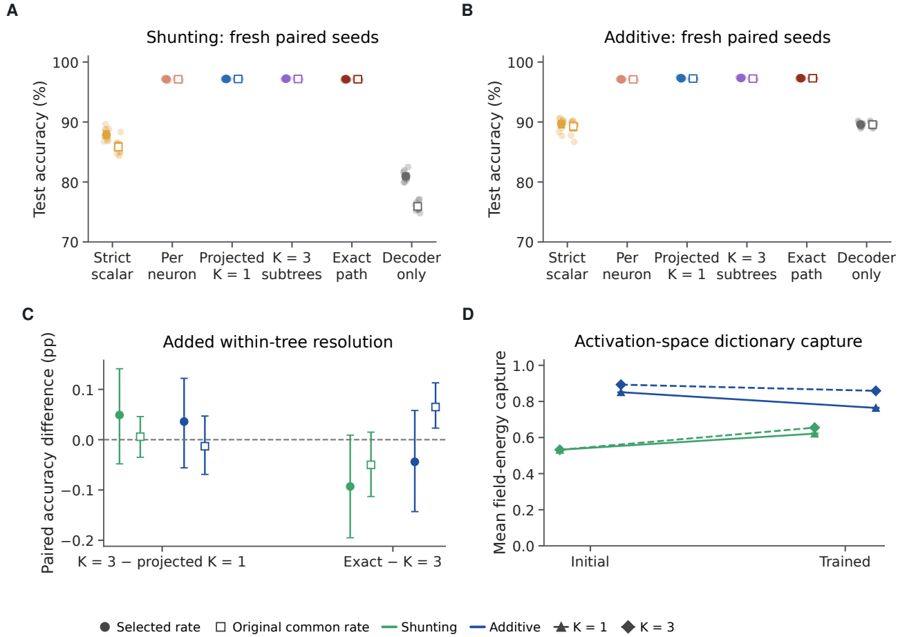
Figure S7: Intermediate dictionaries capture more image-task credit without improving accuracy. A,B , Six-rule MNIST ladder in shunting and raw-additive networks; ten fresh paired seeds per architecture. Filled/open symbols use development-selected/original common rates. Decoder-only learning freezes the initialized core. C , Paired accuracy differences for three profiles versus a projected common profile, and exact versus three-profile credit. D , Initial and trained field-energy capture by uniform K = 1 or subtree K = 3 profiles, averaged over 2,048 held-out images within each seed. Projection coefficients use the exact activation-error field of this ten-seed cohort, so D is not a duplicate of the main-text capture panel; voltage-space capture for the same fits is retained in Source Data. Means and bars in A–D have descriptive 95% seed-bootstrap intervals. Greater capture did not yield an image accuracy benefit. All image cohorts have one dendritic layer and a linear readout.
