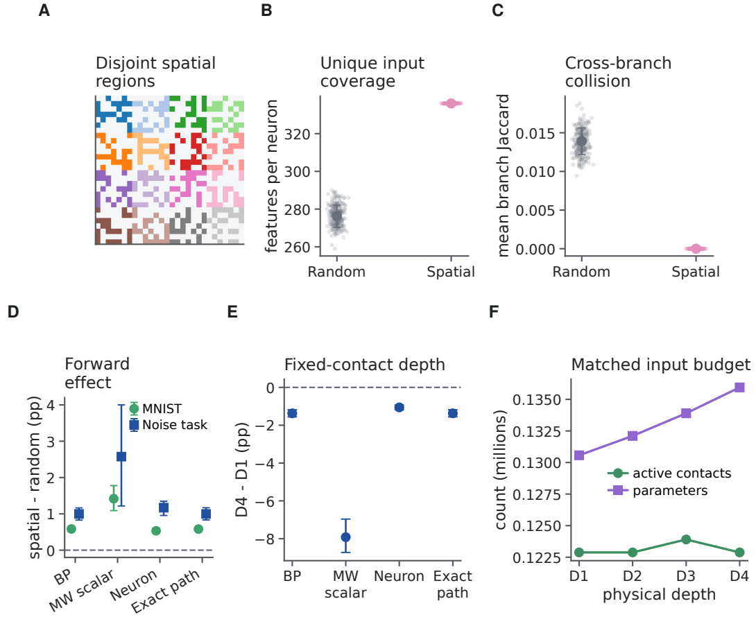
Figure S9: Input coverage and ordinary-task depth are distinct from credit resolution. A–D , Spatial versus randomly assigned contacts in depth-four [2, 2, 2, 2] trees: example map, unique input coverage, cross-branch overlap and learning benefit under backpropagation and three local fields. Contact count is matched, but spatial maps reach more unique inputs and avoid collisions. The accuracy benefit persists under backpropagation and therefore reflects a forward sparsity prior. E,F , Separate raw-additive historical noise cohort with sixteen terminals: all four D4-minus-D1 accuracy contrasts are negative in 10/10 paired seeds; active contact counts are approximately fixed while parameter counts vary. Learning contrasts use means and 95% paired-seed bootstrap intervals; map summaries use mean \pm s.d. The noise-task executed generator remains unresolved and its shunting runs fail the positive-conductance input criterion. These retained additive outcomes are a depth boundary, not evidence for shunting; exclusions are enumerated in Table S5.
