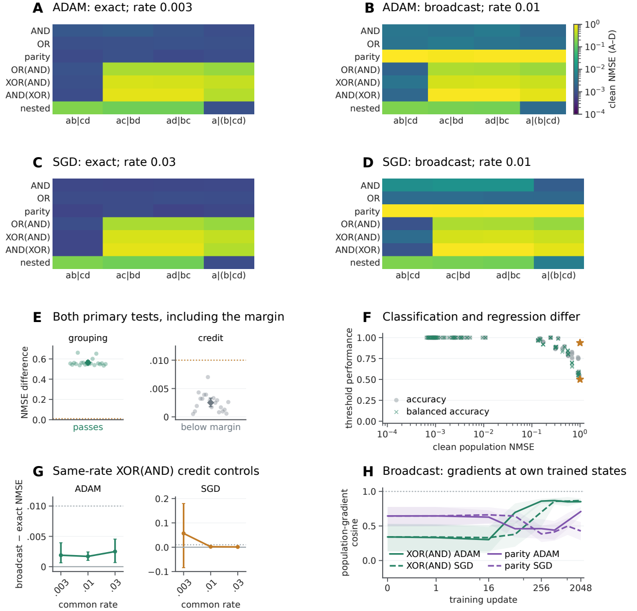
Figure S15: Boolean grouping benefit and a small primary credit effect under frozen recipes. A–D , Clean population normalized mean squared error (NMSE), averaged over twenty fresh seeds: Adam exact ( A ), Adam broadcast ( B ), stochastic gradient descent (SGD) exact ( C ) and SGD broadcast ( D ). Heatmaps share a logarithmic scale; columns show three balanced groupings and one nested tree. Rates were fixed on five development seeds; seeds vary permutations, initialization and noisy observations. E , Prespecified Adam XOR-of-AND contrasts: mean crossed-minus-aligned exact-credit error and aligned broadcast-minus-exact error. Dots, twenty paired seed differences; diamonds/whiskers, means and Bonferroni-adjusted 97.5% intervals (10,000 seed-bootstrap draws). Dotted lines: 0.01-NMSE mean-effect margin. Grouping passes both criteria; the positive credit difference is below the margin. Both compatible rules classify all sixteen patterns perfectly in every seed. F , Accuracy (gray) and balanced accuracy (green) versus NMSE for 112 condition means. Raw-output classification threshold: 0.5. Orange stars show the AND/OR constant-majority references: NMSE one, accuracy 15/16 and balanced accuracy 1/2. G , Same-rate credit contrasts on aligned XOR-of-AND trees, with descriptive 95% intervals; Adam and SGD axes have different ranges. The uncertain low-rate SGD result is retained. H , Broadcast gradient cosine on the aligned balanced tree for XOR-of-AND (green) and parity (purple), with solid Adam and dashed SGD curves, evaluated on all sixteen clean patterns at each learner’s own state, before clipping or optimizer transformation. Bands are pointwise 95% seed-bootstrap intervals. The large parity credit effect is descriptive. All 6,720 fits and 53,760 checkpoints are retained.
