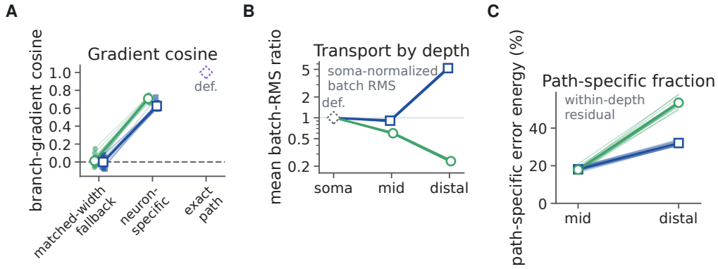
Figure S8: Error-field geometry separates direction, amplitude and spatial variation. Independent fifteen-seed flattened-MNIST cohort of 128 directed [3,3] trees; green circles denote shunting and blue squares raw-additive trees. A , Branch-gradient cosine with the exact gradient at common fixed checkpoints trained with per-neuron feedback; matched-width scalar-fallback and per-neuron fields are evaluated at identical weights and states, and the exact-path cosine of one is definitional. B , Exact voltage-error magnitude by depth at exact-path checkpoints: the batch root-mean-square ratio \text{RMS}(\delta_{n,u}^V)/\text{RMS}(\delta_{0,u}^V) , averaged over neurons and paths, with somatic value one by normalization. C , Within-depth path-specific residual error energy after subtracting the mean across paths within depth d : distal shunting attenuates magnitude but retains the larger path-specific fraction, rising from 18% to 53% (shunting) and 32% (raw additive). Symbols and bars are means and 95% seed-bootstrap intervals. No additional models are trained here; greater path-specific variation did not yield an image accuracy benefit, and voltage- and activation-space capture are different quantities.
