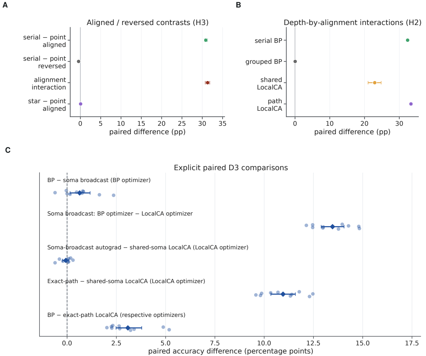
Figure S24: Physical-depth conclusions depend on sensor fidelity, task hierarchy and optimization. A , Serial/point contrasts under matched and reversed sensor placement. B , Separate independently seeded two-level task with D1 [8] and D2 [4, 1]: depth-by-placement interactions for serial and grouped-point backpropagation and for shared or exact-path LocalCA. C , Original-budget D3 optimizer/credit-coordinate contrasts in the serial conductance morphology [2, 1, 2]. Under the BP optimizer, full versus soma-broadcast differentiation differs by 0.64 points; under the split LocalCA optimizer, exact versus shared differs by 10.96 points; changing the broadcast optimizer costs 13.47 points. Means and intervals use ten paired seeds and 95% bootstrap intervals; panel C is generated from source_data/physical_depth_followup/ and is registered in the Source Data manifest. These earlier recipe-specific effects do not imply a converged credit advantage: at 600 epochs the LocalCA accuracy difference reverses, while exact credit retains lower cross-entropy (main Fig. 6). All D3 continuations hit the cap; D1 usually stops early.
