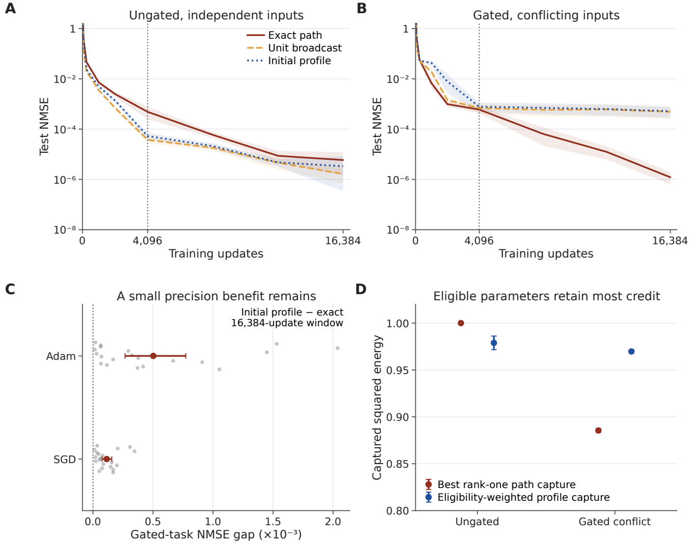
Figure S19: A first conductance task produces a small precision benefit from exact credit. A,B , Test normalized mean squared error (NMSE) at fixed checkpoints under Adam, for ungated independent inputs and gated conflicting inputs in the 16-conductance model. Curves show means and 95% paired-seed bootstrap intervals across 20 fresh seeds; the vertical dotted line marks the original 4,096-update budget. All fits continue to 16,384 updates with unchanged optimizer and minibatch state. Unit and calibrated profiles differ here because global gradient clipping can break Adam’s invariance to fixed positive coordinate scaling. C , Gated-task NMSE differences between the initial calibrated profile and exact credit, evaluated at each fit’s best validation checkpoint in the extended window. Points are paired seed differences; symbols and bars show their means and 95% bootstrap intervals. The Adam gap is 0.000502 [0.000267, 0.000772], positive in all 20 seeds; under Adam, mean broadcast error nevertheless remains below 0.0006 NMSE. D , Diagnostics at the exact-rule best-validation states distinguish the best rank-one capture of the six-compartment path field from capture by each student’s fixed initial profile after weighting by local parameter eligibility. Both are squared-energy projection ratios with one freely fitted amplitude per example. High eligibility-weighted capture helps explain the small learning difference. The gated and ungated tasks change both inhibition and distractor dependence, so this first study is a task-family comparison. All 216 development fits, 240 fresh fits and their continuations are retained in Source Data.
