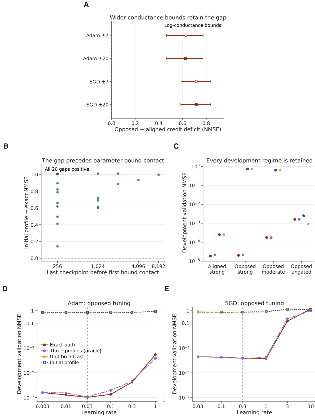
Figure S20: Parameter-range, development and rate controls retain the opposed-task broadcast deficit. A , Task-by-credit interaction under original [-7, 7] and wider [-20, 20] log-conductance bounds, with Adam and SGD. All fits retain their original initialization/minibatch streams and extend to 16,384 updates; endpoints use validation-selected checkpoints. Wider-bound interactions are positive in all seeds. B , Initial-profile-minus-exact NMSE at each seed's last saved checkpoint before that seed's calibrated-profile fit first reaches an original bound; all twenty differences are already positive. Dots are twenty paired seeds and intervals are 95% paired bootstrap intervals in A,B . C , All four retained development regimes under Adam, using each rule's lowest mean validation NMSE among its three equally budgeted rates: aligned strong gating, opposed strong gating, opposed moderate gating (inactive-parent inhibitory activity one) and opposed ungated (activity zero). These are development summaries over three seeds, not additional confirmatory seed blocks. D,E , Equally budgeted six-rate development sweeps for opposed tuning under Adam and SGD; corresponding aligned-task outcomes are retained in the full condition table and in Source Data rather than drawn here. Each point averages three development seeds; all 288 outcomes are retained. The predefined improvement trigger was not reached, so rates were not retuned on fresh test outcomes. Some broadcast fits also reach wider bounds; these are finite-budget controls, not an asymptotic convergence proof.
