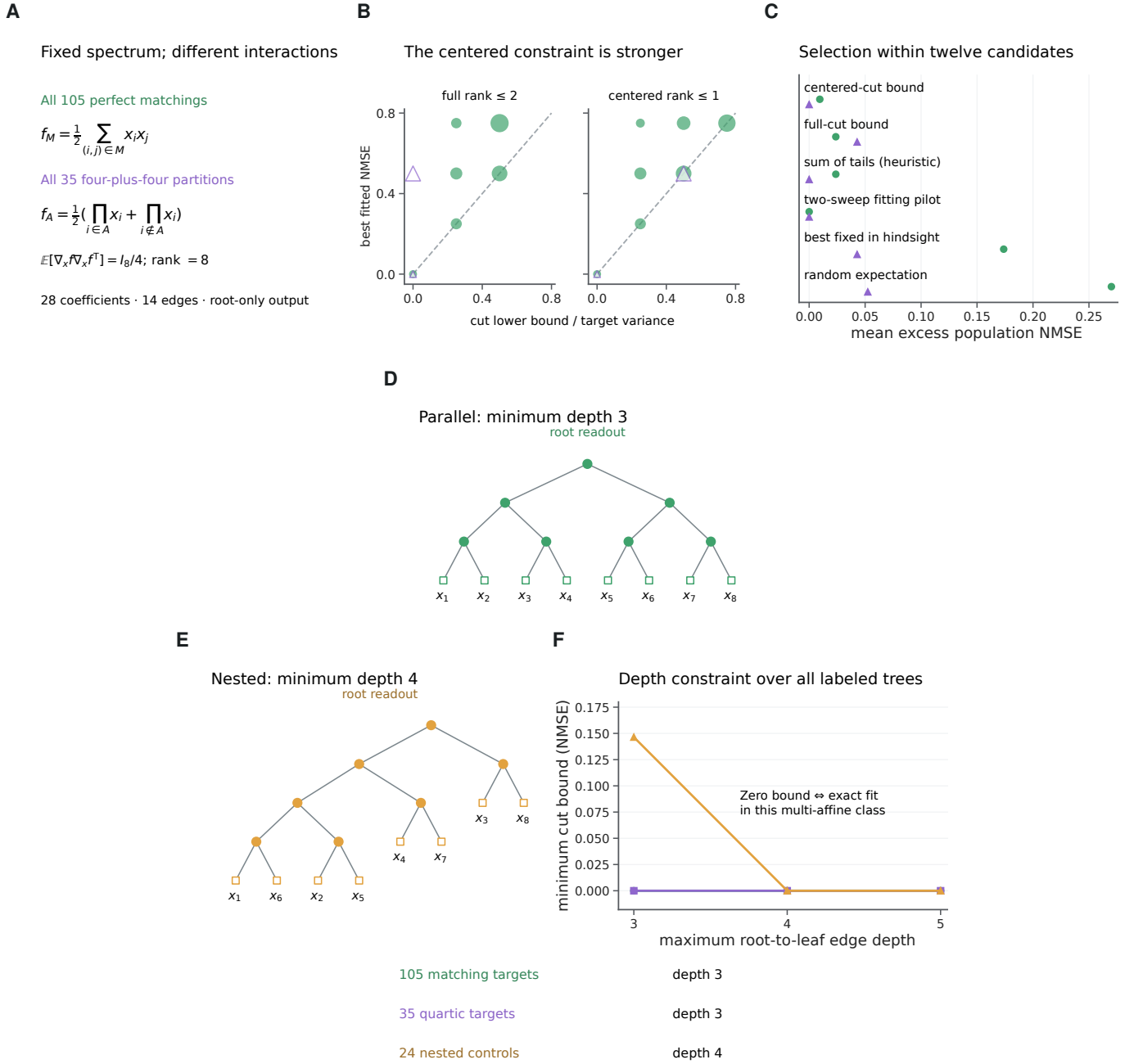
Figure S12: Interaction structure constrains scalar trees at matched input spectra and resources. A , Exhaustive pairwise matching and two-quartic target families on eight independent binary inputs; both have input-gradient second moment I_8/4 . Each candidate has seven scalar multi-affine nodes, 28 coefficients and fourteen edges. B , Full rank-two and centered rank-one cut-tail lower bounds versus achieved population NMSE in four-restart alternating least squares. C , Mean excess NMSE above the best fitted candidate in the fixed pool of twelve; score ties use tolerance 10^{-10} and lexicographic candidate identifier, and best-fixed selection uses family outcomes in hindsight. D , Actual tree returned for the first enumerated matching, a depth-three parallel construction. E , First seeded nested-prefix control tree, of minimum depth four. Leaves access the indicated input only. F , Minimum possible maximum centered-cut bound over all labeled binary trees at each depth limit, calculated separately for every target: matching and quartic targets admit exact depth-three trees, whereas nested controls require depth four and do not share the I_8/4 input spectrum. The key below the panels gives the target counts and minimum exact depths of the three families. All 164 targets construct with error below 7 \times 10^{-30} and coefficients of magnitude at most one. These exhaustive capacity results have no sampling error bars. The theorem concerns scalar multi-affine composition, not arbitrary conductance dendrites.
