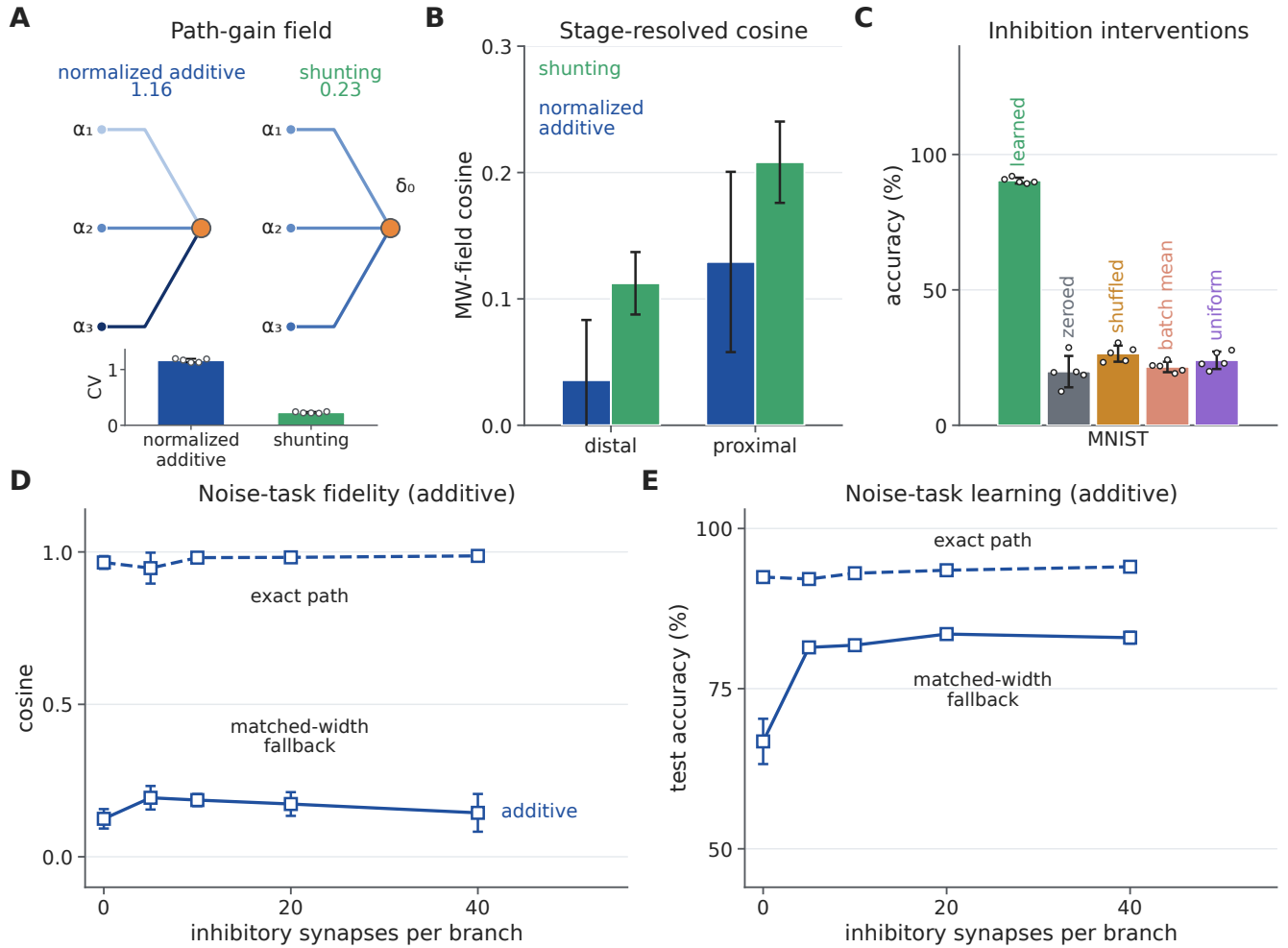
Figure S1: Mechanistic chain from path gains to learning in regular-tree models. MNIST panels A–C use two-stage [4, 4] directed trees; the historical noise-resilience panels D, E use two-stage [3, 3] additive trees. A , Conductance-stage path-gain field in shunting and normalized-additive models at five inhibitory synapses per branch; the inset shows paired-seed coefficients of variation (CV; standard deviation divided by mean). The displayed \alpha values are path gains and \delta_0 is the somatic error. This loading quantity omits branch derivatives and is distinct from the trained exact-error profiles in Supplementary Fig. S8B, C. B , Stage-resolved cosine of matched-width scalar fallback versus exact MNIST errors; the width-matched somatic stage is excluded because its cosine is one by construction. C , MNIST post-training inhibition interventions: zero, sample shuffle, per-branch batch mean and a uniform matched mean. These also change forward computation and do not isolate backward shunting. D, E , Feedback fidelity and learning on the additive noise task; solid and dashed lines denote matched-width scalar-fallback and exact transport. Bars show standard deviations across checkpoints in B and retained runs in C–E ; white points in C identify runs. Historical noise-task shunting aggregates with unresolved execution lineage are excluded and retained in Source Data only. The retained additive aggregates do not resolve their normalization setting. The state-matched focal analysis in main Fig. 8 provides the conductance-specific transport comparison. This chain is the figure support for Supplementary Section S1; the exact-path field it feeds is drawn at the main-text type scale in main Fig. 1.
