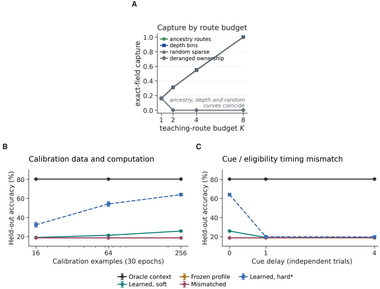
Figure S11: Available route span and learned route coefficients are different constraints. A , Trained field capture by route budget in the eight-context factorial. Ancestry, depth and random partitions have coincident capture at matched bandwidth; derangement removes the target coordinate. Capture therefore does not explain the small ancestry-specific advantage, and capture alone does not predict trained utility: the within-seed Spearman correlation between capture and utility is about 0.82 over all budgets and 0.64 for K < 8 , and is retained numerically in Source Data. B , Held-out accuracy versus calibration set size (16, 64 and 256 examples) at cue-noise standard deviation 0.5 and zero delay; 30 epochs are fixed, so both data and computation increase. C , Cue delay at 256 calibration trials and noise SD 0.5; delays mismatch independent contexts and are measured in trials, not physiological time. In B,C the dashed curves marked with an asterisk use maximum-probability route selection by the same frozen encoder, an exploratory paired sensitivity specified after the soft outcomes with no encoder refit. Curves, diamonds and bars are means and 95% paired-seed bootstrap intervals over twenty fresh analysis seeds. The cue-noise sensitivity of the same encoder is drawn at the main-text type scale in main Fig. 3F. The calibration cue and activation targets are supplied resources. No serial forward dendritic computation is present.
