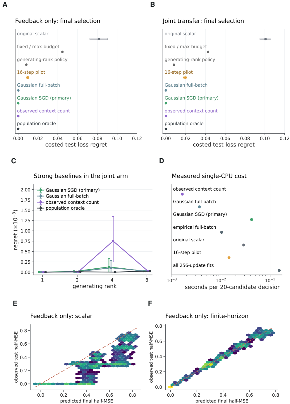
Figure S35: Finite-horizon prediction improves selection but strong simple baselines remain. A,B , Final costed-test-loss regret by imposed rank in the feedback-only and joint-transfer fixed-cache learners; regret is excess above the best trained candidate. C , Differences among strong selectors at each rank in the joint arm. The independently calibrated Gaussian SGD forecast improves over the original scalar utility; the full-batch and observed-context-count baselines remain competitive. All finite-horizon policies choose K = r in this family, so improvement does not establish fine morphology selection. D , Median measured elapsed time on one central processing unit per twenty-candidate decision. Plug-in timings include calibration-model preparation, count-only time excludes shared calibration generation, and the pilot includes sixteen candidate updates; times measure these implementations, not hardware-independent complexity. E , Original scalar forecast versus final test half-mean-squared-error in the feedback-only arm. F , The calibration-derived Gaussian SGD forecast on the same cases and arm. Hexagons encode counts on a logarithmic color scale and dashed lines mark equality; the joint arm reproduces E,F and is retained in Source Data. The population-oracle forecast bias — predicted minus exact population loss of the realized trained weights under fresh examples or finite-cache reuse — is retained in Source Data: the fresh-example recurrence is exact under the stated Gaussian and conditional-linear assumptions, whereas cache reuse violates independence. Curves and whiskers in A–D are means and pointwise 95% intervals from 10,000 whole-seed bootstrap draws over twenty seed blocks. All 25,600 candidate fits and both regimes are retained. These are linear-learning forecast tests, not a general nonlinear dendritic morphology law.
