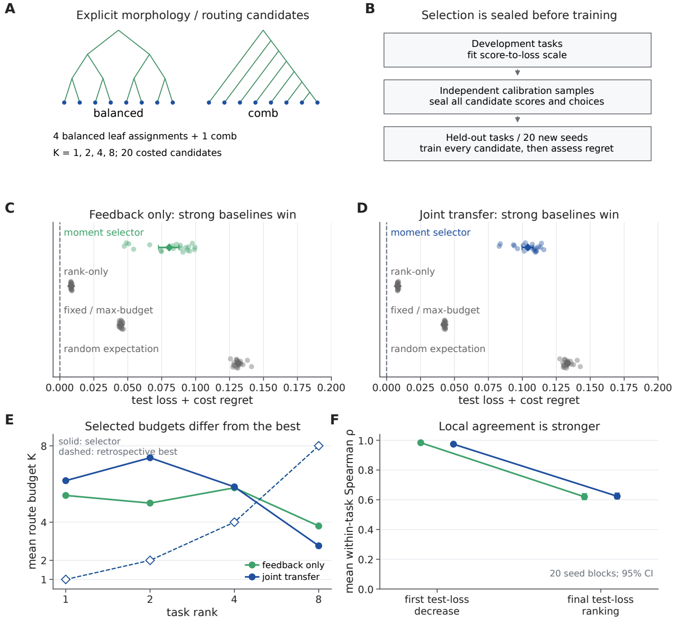
Figure S34: The original scalar initialization score predicts a first step but fails at prospective endpoint selection. A , Four balanced leaf assignments and one comb supply route budgets K = 1, 2, 4, 8 : twenty candidates with prescribed cost; K counts feedback channels. B , Development, independent calibration, sealed choices and confirmation training. C,D , Final test half-mean-squared-error (MSE) plus cost, expressed as excess over the best trained candidate, for feedback-only and joint passive-transfer arms, respectively. Small points are twenty whole-seed means; diamonds and whiskers are means and 95% seed-bootstrap intervals (10,000 draws). The development-fixed/max-budget and privileged generating-rank baselines outperform the moment selector; random expectation averages all candidates uniformly. E , Selected mean budget versus imposed rank; dashed curves show the retrospectively best candidate's budget. F , Mean within-task Spearman correlation of initialization utility with actual first-step test-loss decrease and final test-loss ranking. Intervals resample whole seeds. All 12,800 confirmation candidate fits and 38,400 checkpoints remain included. Every model has a freely trained dense weight matrix; passive transfer changes conditioning and cost but does not necessarily restrict representation. This experiment is distinct from the locally connected multi-affine construction and the separately frozen finite-horizon follow-up.
