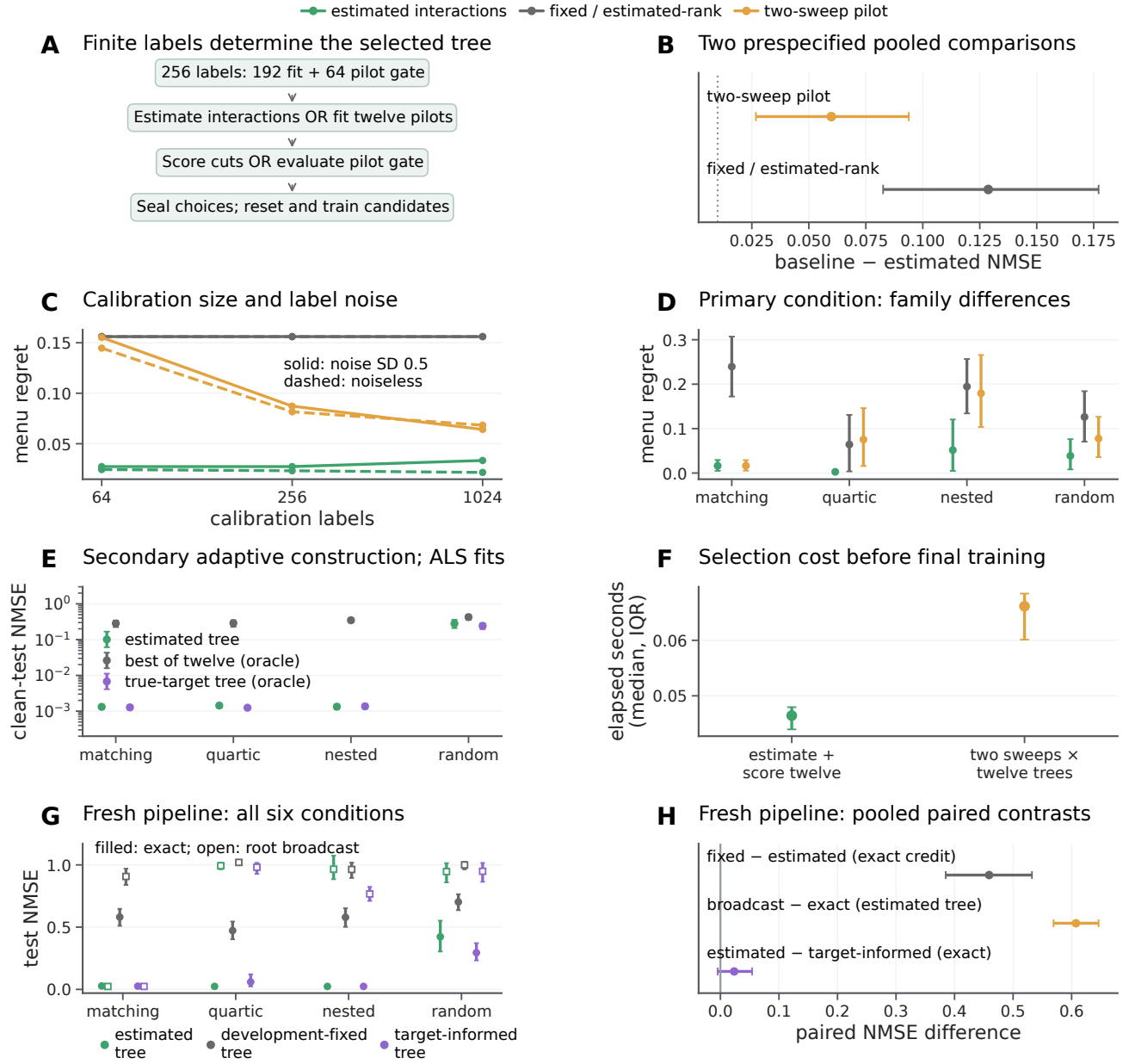
Figure S36: Finite calibration, adaptive construction and direct gradient learning. A , Primary calibration: 256 labels, noise standard deviation (SD) 0.5; 192 observations for estimation/pilot fitting and 64 for pilot gating. The 255-term Walsh estimator receives no family labels, true support or coefficients. The pilot fits all twelve candidates for two sweeps. Choices are sealed; training restarts independently. B , Prespecified pooled fixed-baseline-minus-estimated and pilot-minus-estimated normalized mean squared error (NMSE). Whiskers are Bonferroni-adjusted 97.5% paired bootstrap intervals; the dotted line marks the 0.01-NMSE meaningful-improvement margin. C , Excess clean-test NMSE above the best trained candidate across calibration sizes; solid curves use noise SD 0.5 and dashed curves no noise. D , Family-specific primary regret for estimated interactions, the development-fixed/estimated-rank baseline and the fitting pilot; pooled superiority is not uniform across families. E , Secondary adaptive trees trained with alternating least squares (ALS), versus the best trained twelve-candidate menu and a full-target construction oracle. Random-interaction errors remain. F , Elapsed time (median and interquartile range) on one CPU for eighty tasks: estimation/scoring of twelve trees versus pilot fitting/gating, excluding final training. G,H , Independent twenty-seed Adam cohort. G , Three structures and two credit rules in four non-isospectral families: filled symbols, exact credit (Adam 0.01); open, root broadcast (0.003). Label-noise floor: 0.0225; E uses clean targets. H , Fixed-minus-estimated error under exact credit and broadcast-minus-exact error on estimated trees use Bonferroni-adjusted 97.5% intervals; estimated-minus-target-informed error under exact credit uses a pointwise 95% interval. Target-informed construction is not a performance ceiling. Other whiskers: pointwise 95% intervals, 10,000 whole-seed bootstrap draws ( n = 20 ); pooled statistics average families within seed. Both cohorts are independent of Supplementary Fig. S13.
