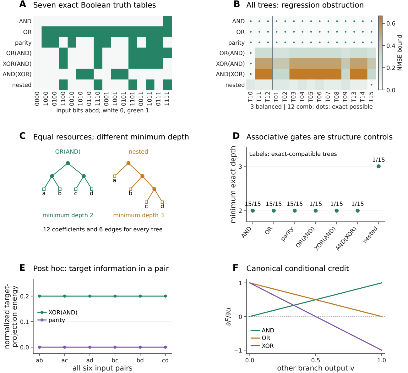
Figure S14: Boolean interactions distinguish structure, depth and canonical credit. A , Complete truth tables of seven four-input templates, with sixteen equally weighted patterns (white, 0; green, 1). Mixed targets are (a \wedge b) \vee (c \wedge d) , (a \wedge b) \text{ XOR } (c \wedge d) , (a \text{ XOR } b) \wedge (c \text{ XOR } d) , and nested a \wedge [b \vee (c \wedge d)] . B , Centered-cut normalized-mean-squared-error (NMSE) regression lower bounds for all fifteen labeled binary trees. Green dots mark 49 exactly representable family–tree pairs, independently certified with coefficients in [-2, 2] . The largest coefficient magnitude in these constructions is 4/\sqrt{15} . All trees have twelve coefficients and six edges; T identifiers and cut sets are supplied in Source Data. A positive bound concerns truth-value regression, not threshold classification. C , OR-of-AND and the nested function each use two AND gates and one OR gate, but require minimum exact depths two and three. D , Minimum exact depth and compatible-tree counts. AND, OR and parity admit all fifteen trees; each mixed-gate target admits one. All seven input-sensitivity matrices have rank four, but their spectra generally differ. E , Explicitly post hoc target-projection energy \|\mathbb{E}[z | x_S]\|^2 for all six two-input subsets, with normalized target z . Parity has zero energy on every proper subset; XOR-of-AND has energy 1/5 on every pair, including crossed pairs. This describes local target information and does not predict grouping compatibility or prove broadcast-learning failure. F , Canonical derivatives \partial F / \partial u with respect to left-branch output u , versus right-branch output v : AND, v ; OR, 1 - v ; XOR, 1 - 2v . These raw Boolean coordinates are illustrative; training can change every coefficient and need not preserve them. No learning outcome is inferred from a derivative sign alone. Panels are exhaustive analytic diagnostics, with no sampling error bars; the multi-affine and independent-input assumptions are explicit in Supplementary Note 4.4.
