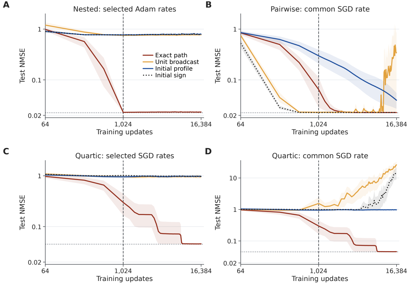
Figure S17: Nested targets and SGD controls in the balanced budget extension. A , Nested targets at selected Adam rates. B , Pairwise targets at the common SGD rate. C,D , Quartic targets at selected and common SGD rates. The same previously observed twenty seeds, fixed rules and rate choices are retained. Curves show mean test NMSE from update 64 onward; bands give descriptive 95% whole-seed bootstrap intervals. Vertical lines mark the original 1,024-update cap and horizontal lines the relevant noise floor. Panels state the task, optimizer and rate view; no outcome is excluded or used to retune rates. These controls retain optimizer dependence and bounded-parameter scope.
