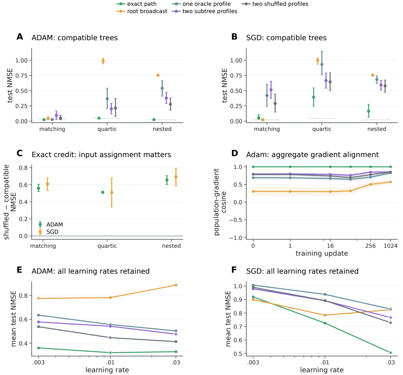
Figure S13: Task-dependent credit requirements in bounded multi-affine trees. A,B , Final test normalized mean squared error (NMSE) on oracle-compatible trees under Adam and stochastic gradient descent (SGD), respectively. Exact path, root broadcast, one oracle profile, two subtree profiles and two shuffled profiles share the forward model, initialization, examples and minibatches. Dotted segments mark known label-noise floors: 0.0225 for matching/nested tasks and 0.045 for quartic tasks. Projection coefficients access the exact current path field and are oracle diagnostics; root broadcast supplies the same scalar error to each internal node. C , Paired exact-credit NMSE increases after shuffling leaf input assignments while preserving tree shape and parameter count. Chance-compatible shuffles are retained. D , Adam gradient cosine between the exact and delivered aggregate clean-population updates, evaluated at each rule's own trained state. Each seed averages the three task families before aggregation; these are not comparisons at a common model state or mean per-example cosines. Points and whiskers in A–C and bands in D are means and pointwise 95% intervals from 10,000 whole-seed bootstrap draws, with twenty independent fresh seeds per family. E,F , Final NMSE at all three learning rates, averaged over both compatible and shuffled assignments and all three families. Stars mark rates selected separately for each rule and optimizer using only development seeds. These means therefore differ from compatible-only panels A,B . Every SGD choice was the upper tested rate; the result is a comparison of the stated training recipes, not a fully optimized SGD limit. Matching and quartic tasks share the input-gradient second moment I_8/4 ; nested tasks have a different spectrum. The oracle-compatible architectures here are independent of the noisy morphology-selection experiment. All 3,600 fresh fits and all tested rates are retained. Panel C is reproduced at the main-text type scale as main Fig. 4H.
