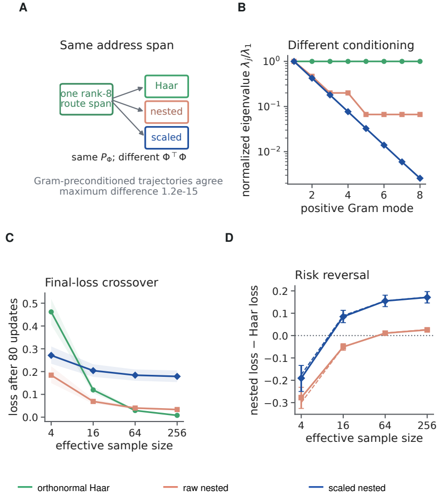
Figure S5: Identical route spans can learn differently through conditioning. A , Haar, redundant nested and statically scaled nested coordinates parameterize the same rank-eight span in sixteen abstract coefficients. B , Positive Gram eigenvalues; condition numbers are 1, 15 and 388.52. C , Population loss after eighty updates across effective sample size. D , Paired nested-minus-Haar contrasts; negative values favor nested coordinates. Points and bars are means and 95% paired-seed bootstrap intervals across fifty seeds; dashed curves are the exact finite-time risk. Slow modes reduce variance at low data and retain bias at high data. Gram-preconditioned controls agree to 1.15 \times 10^{-15} . This is a coefficient-learning comparison within one span, not a simulation of forward dendritic morphology or a biological implementation of the preconditioner.
