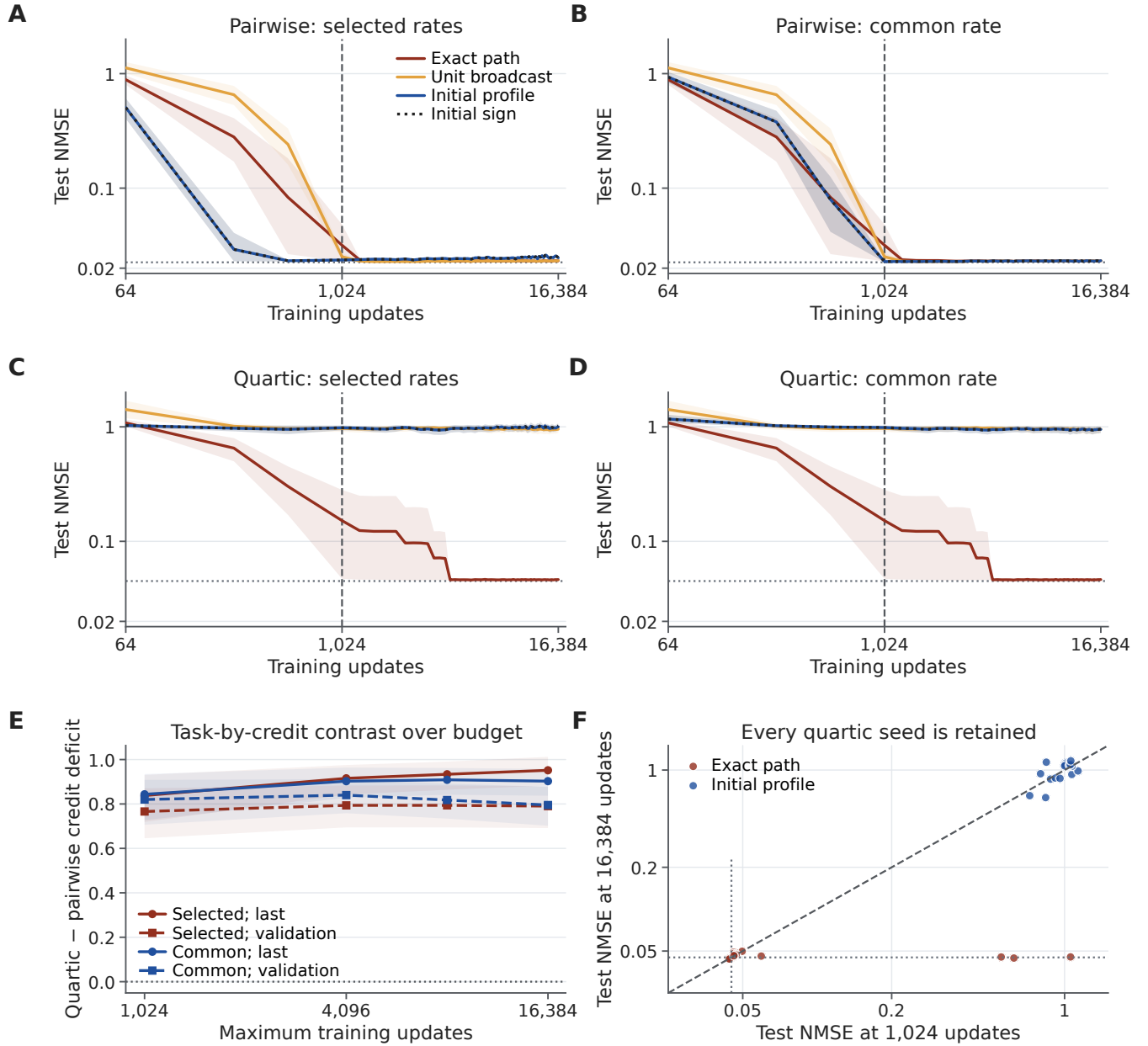
Figure S16: Longer matched budgets retain the task-dependent fixed-profile deficit. A,B , Pairwise targets under Adam at the separately selected rates and at the common rate, with exact, unit-broadcast, initial-profile and initial-sign credit. C,D , Quartic targets at the same two rate choices. Initial-sign controls use dotted curves; vertical lines mark 1,024 updates and horizontal lines mark noise-only NMSE. E , Quartic-minus-pairwise difference in calibrated-minus-exact NMSE across four budgets: circles use terminal states and squares validation-selected states. F , Every exact and calibrated quartic seed at the original 1,024-update and extended 16,384-update endpoints; the diagonal marks unchanged error. Panel F resolves the three stalled seeds that main Fig. 4D draws as individual trajectories. Curves show means and descriptive 95% whole-seed bootstrap intervals. All 720 trajectories retain the previously observed twenty seed blocks, three tasks, four rules, two optimizers and the union of the original selected and common rates. The complete original endpoints replay exactly. Slow exact quartic fits resolve with more updates; restricted profiles retain a large deficit. Rates remain fixed and coefficients bounded; this is a retrospective-cohort extension under a prospective protocol, not fresh confirmation.
