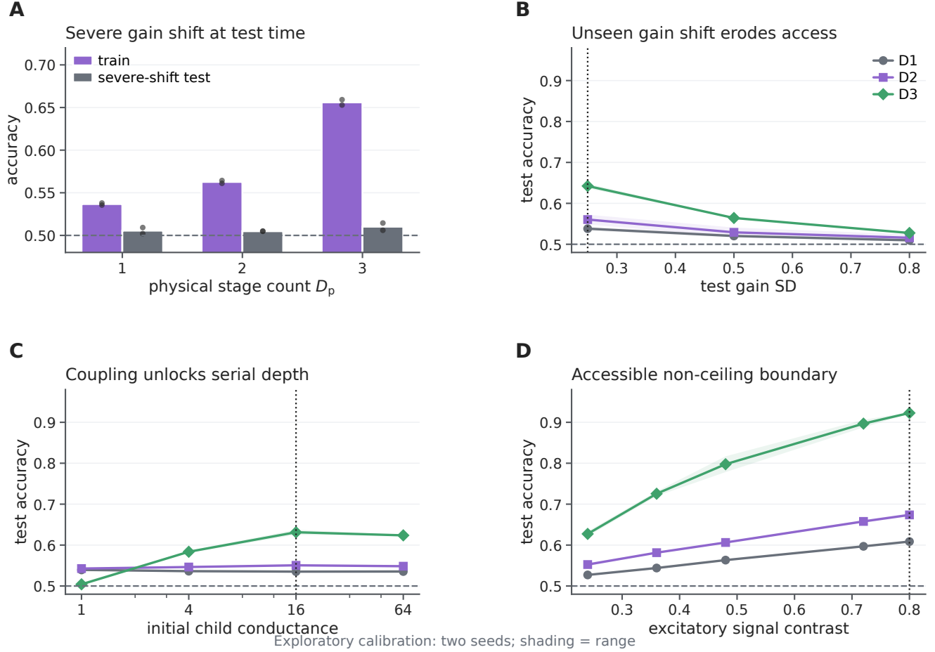
Figure S23: Transparent calibration of the nonlinear physical-depth operating point. All panels use the three-level hierarchical gain-load task and serial shunting morphologies D1 [8], D2 [2,3] and D3 [2,1,2], each with eight nonsomatic compartments per soma. They test the prerequisite for the main hypothesis: whether the mechanism-matched divisive task is accessible at every depth before comparing depth benefits. A , The original aligned shunting-backpropagation (BP) pilot at signal contrast 0.24 fit the training distribution increasingly with depth but remained at chance under the prespecified severe gain shift (test gain standard deviation (SD) 1.2). Bars are two-seed means and dots are the individual exploratory seeds. B , With training gain SD fixed at 0.25, increasing unseen test gain variation eroded accessibility at every depth. The dotted line marks the matched train/test condition. C , At matched gain and signal contrast 0.24, stronger child coupling selectively made serial D3 computation accessible; the dotted line marks child conductance 16 used subsequently. D , At matched gain and child conductance 16, increasing excitatory signal contrast moved D1–D3 away from chance without saturating D1 or D2. The separately run 0.80 boundary (dotted line) met the predefined accessibility criterion and selected the operating point used for the analysis seeds. Lines show two-seed means; shading spans the two exploratory values and is not a confidence interval. All pilot, ladder and boundary seeds were excluded from the confirmatory contrasts.
