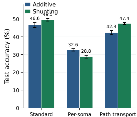
A CIFAR-10 mechanism ladder
